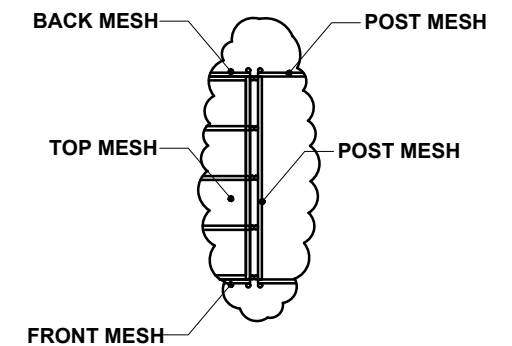
FITTING DETAIL "A"
