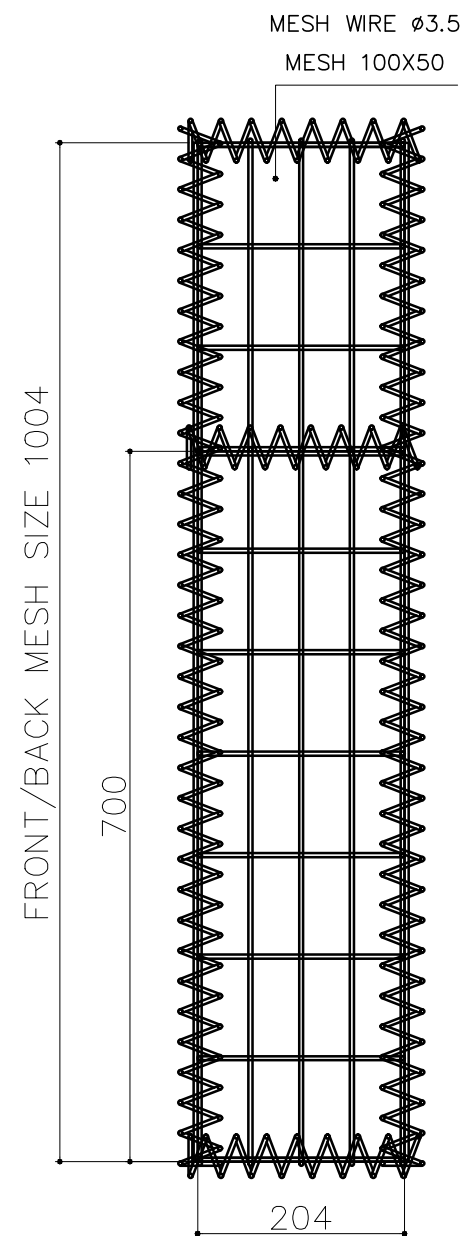
TYPICAL ELEVATION
