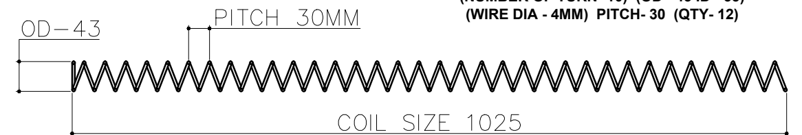
(POST L / R COIL) (COIL LENGTH - 1220) (NUMBER OF TURN- 35) (OD - 43 ID - 35) (WIRE DIA - 4MM) PITCH- 30 (QTY- 04)
