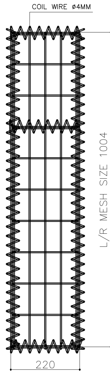
SIDE VIEW
