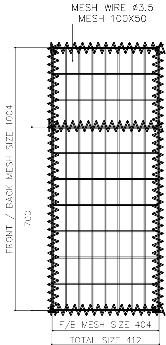
TYPICAL ELEVATION
