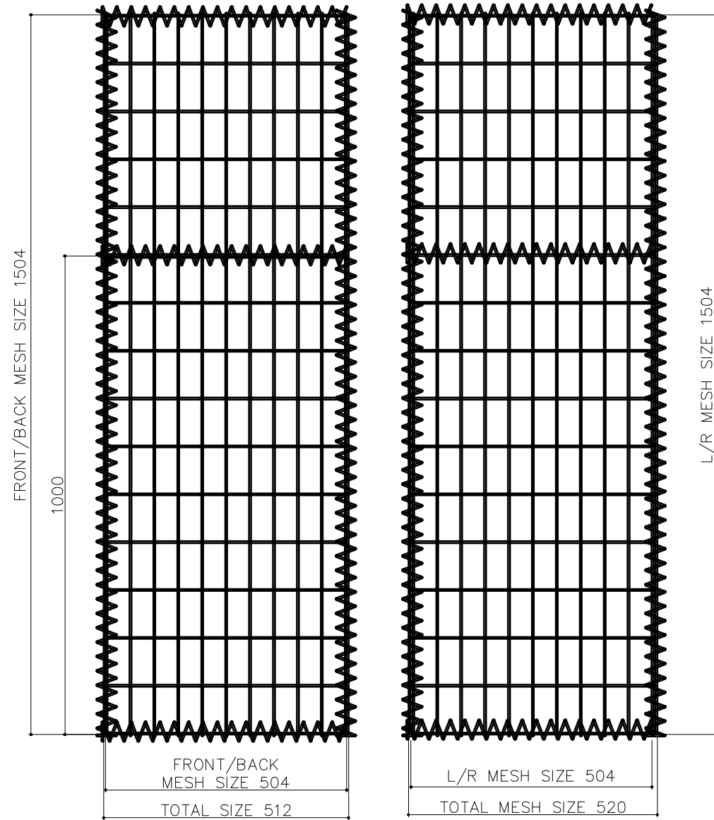
TYPICAL ELEVATION
