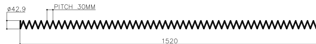
(POST L / R COIL) (COIL LENGTH - 1520) (NUMBER OF TURN - 52) (OD - 43 ID - 35) (WIRE DIA - 4MM) PITCH - 30 (QTY - 04)
