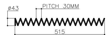
(POST TOP/BOTTOM COIL) (COIL LENGTH - 515) (NUMBER OF TURN - 18) (OD - 43 ID - 35) (WIRE DIA - 4MM) PITCH - 30 (QTY - 08)
