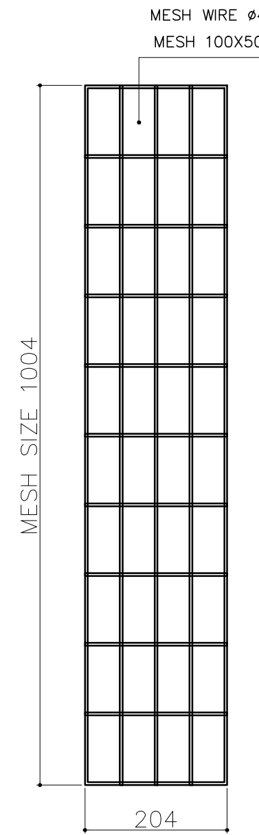
FRONT / BACK / LEFT / RIGHT MESH MESH SIZE 100X50 (QTY-04)
