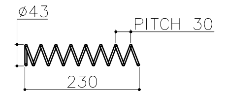
(POST TOP/BOTTOM COIL) (COIL LENGTH - 230) (NUMBER OF TURN- 10) (OD - 43 ID - 35) (WIRE DIA - 4MM) PITCH- 30 (QTY- 12)
