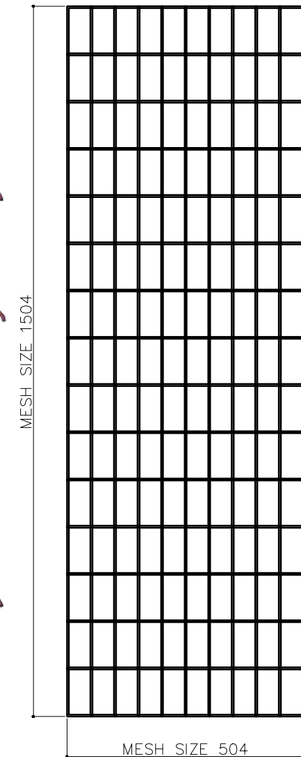
FRONT / BACK / LEFT / RIGHT MESH MESH SIZE 100X50 (QTY-04)
