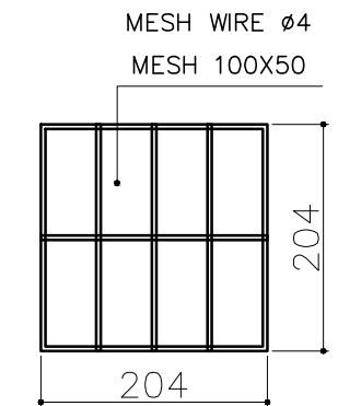
POST TOP / BOTTOM / CENTER MESH MESH SIZE 100X50 (QTY-03)
