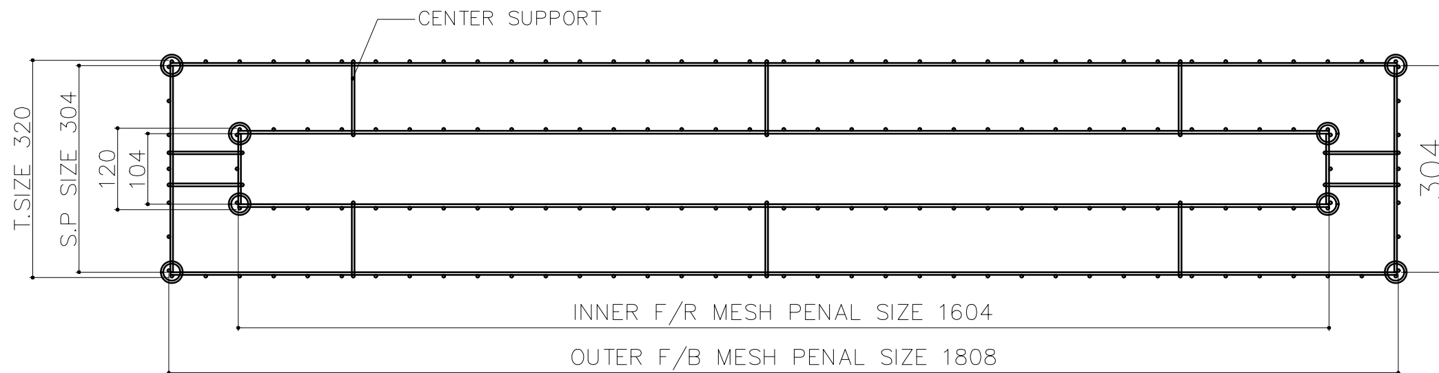
TOP / PLAN
