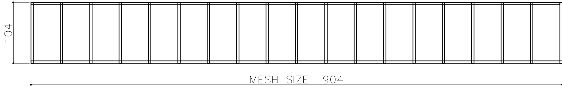
OUTER FRONT / BACK MESH PENAL MESH SIZE 100X50 (MESH WIRE DIA 4MM) QTY-02
