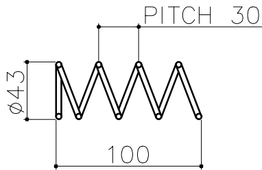
INNER OUTER MESH PENAL COIL NUMBER OF TURN-5 TOTAL LENGTH - 100 WIRE DIA- 4MM (QTY-08)
