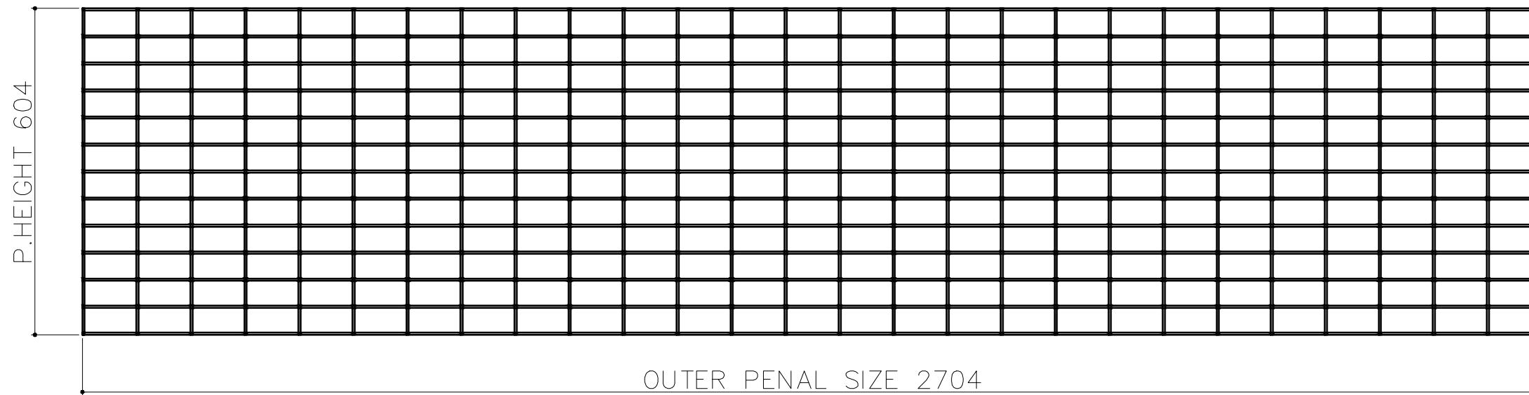
OUTER FRONT BACK MESH PENAL QTY -02 (MESH WIRE Ø4MM) MESH SIZE 100X50
