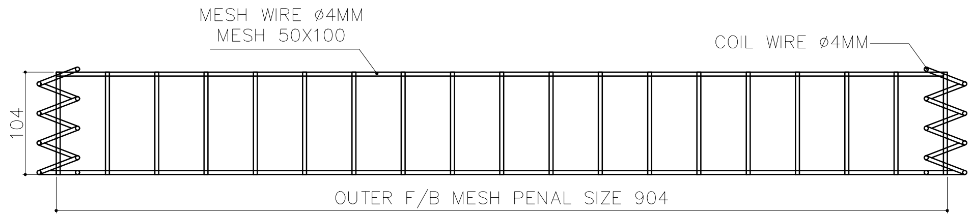
TYPICAL ELEVATION
