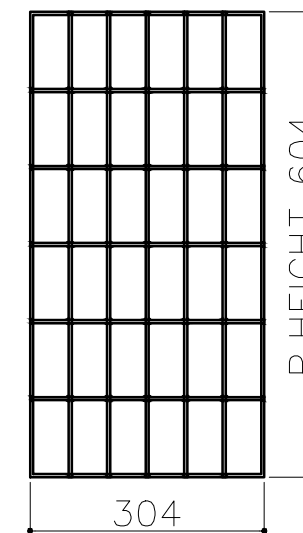
OUTER LEFT / RIGHT MESH PENAL QTY -02 (MESH WIRE Ø4MM) MESH SIZE 100X50
