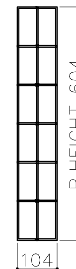
INNER LEFT / RIGHT MESH PENAL QTY -02 (MESH WIRE Ø4MM) MESH SIZE 100X50
