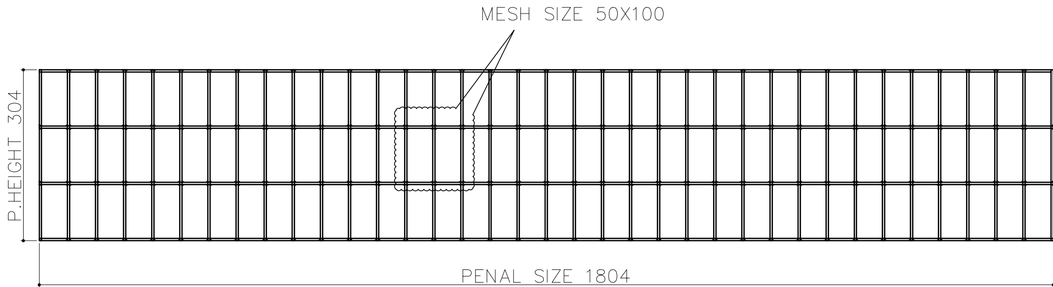
OUTER FRONT BACK MESH PENAL QTY -02 (MESH WIRE Ø4MM) MESH SIZE 100X50
