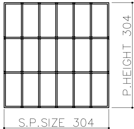
OUTER LEFT RIGHT MESH PENAL QTY -02 (MESH WIRE Ø4MM)
