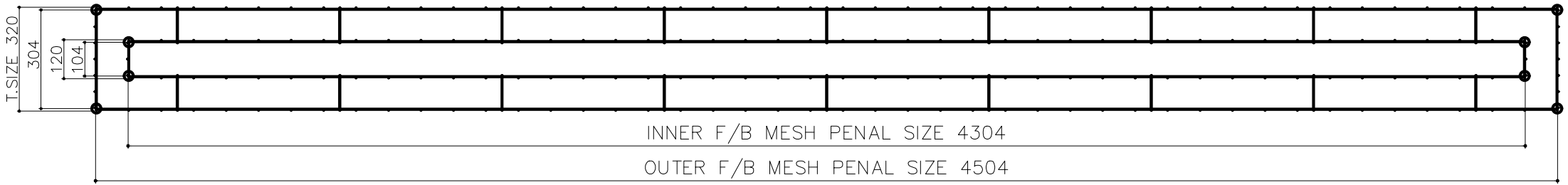
TOP / PLAN
