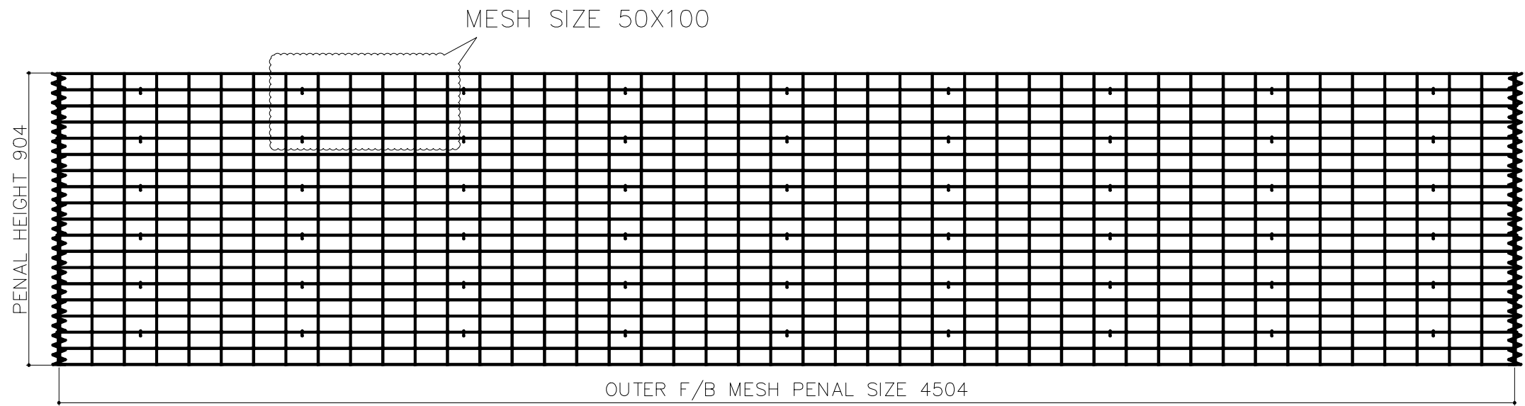
TYPICAL ELEVATION
