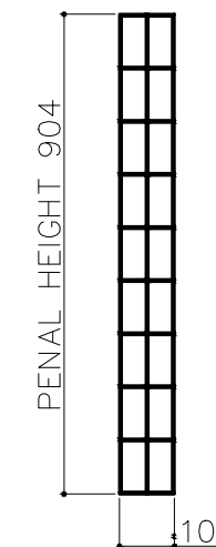
INNER LEFT / RIGHT MESH PENAL QTY -02 (MESH WIRE Ø4MM) MESH SIZE 100X50
