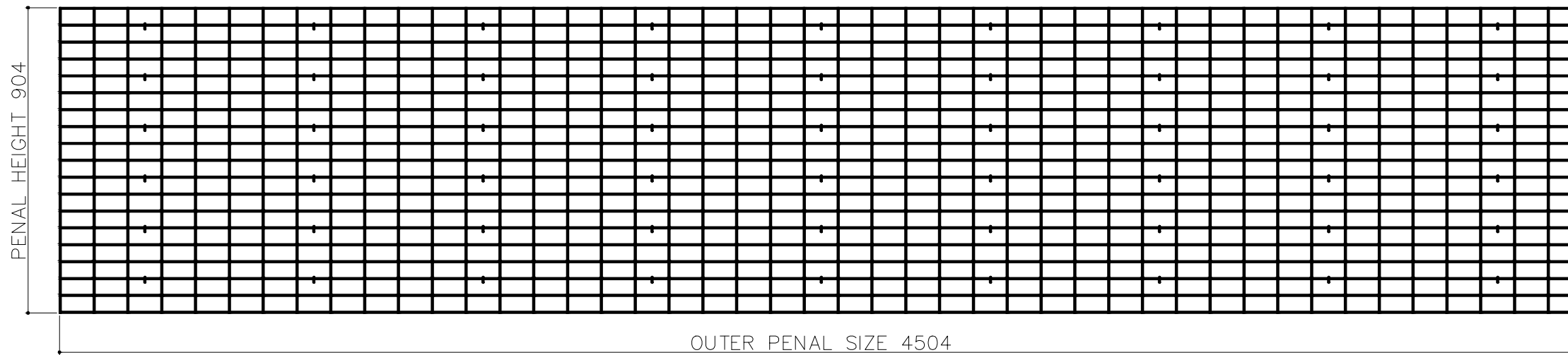
OUTER FRONT BACK MESH PENAL QTY -02 (MESH WIRE Ø4MM) MESH SIZE 100X50
