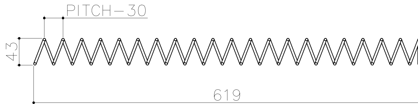
COIL WIRE Ø4MM ID-35 OD-43 NUMBER OF TURN 22 PITCH-30MM (QTY-08)
