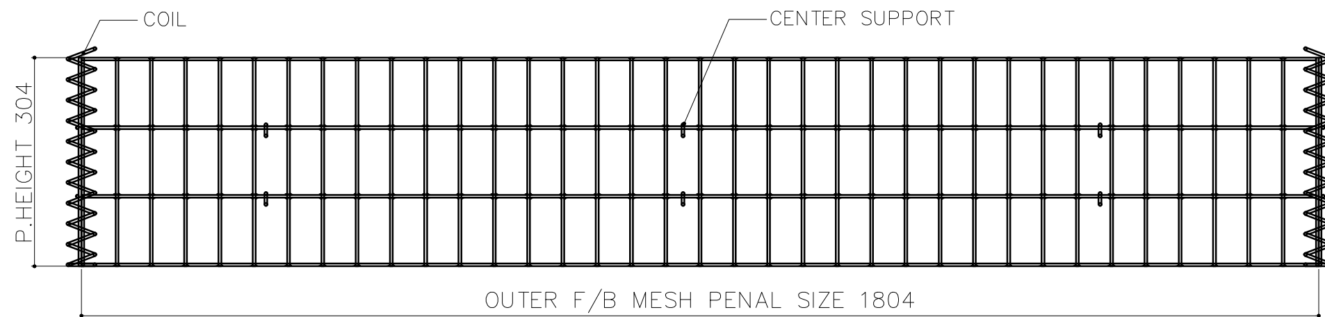
TYPICAL ELEVATION
