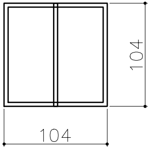
INNER LEFT/ RIGHT MESH PENAL MESH SIZE 100X50 (MESH WIRE DIA 4MM) QTY-02
