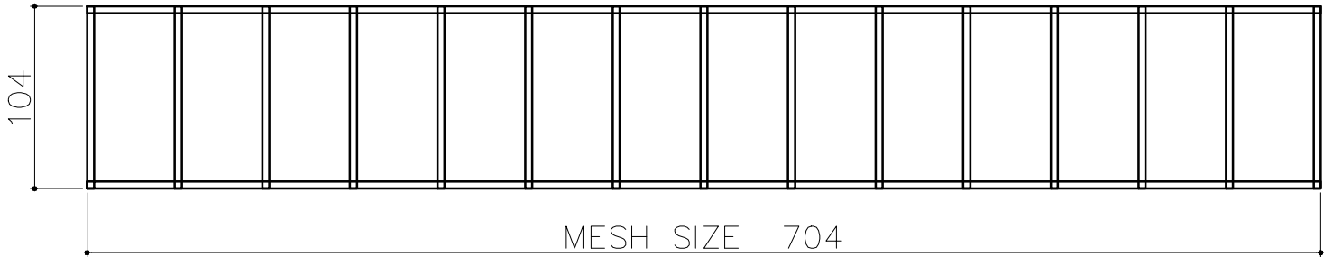
INNER FRONT / BACK MESH PENAL MESH SIZE 100X50 (MESH WIRE DIA 4MM) QTY-02
