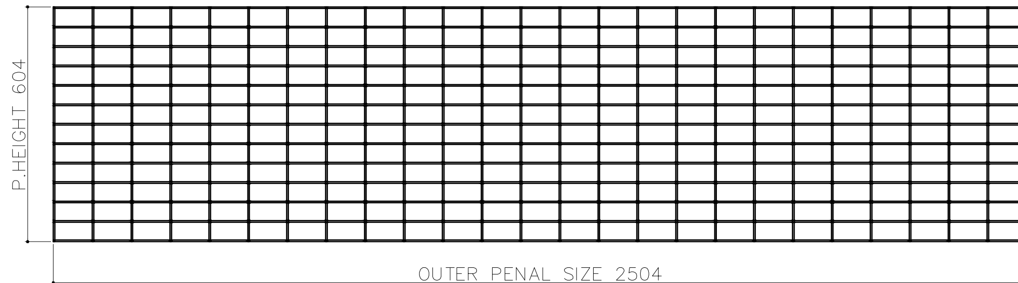
INNER FRONT BACK MESH PENAL QTY -02 (MESH WIRE Ø4MM) MESH SIZE 100X50
