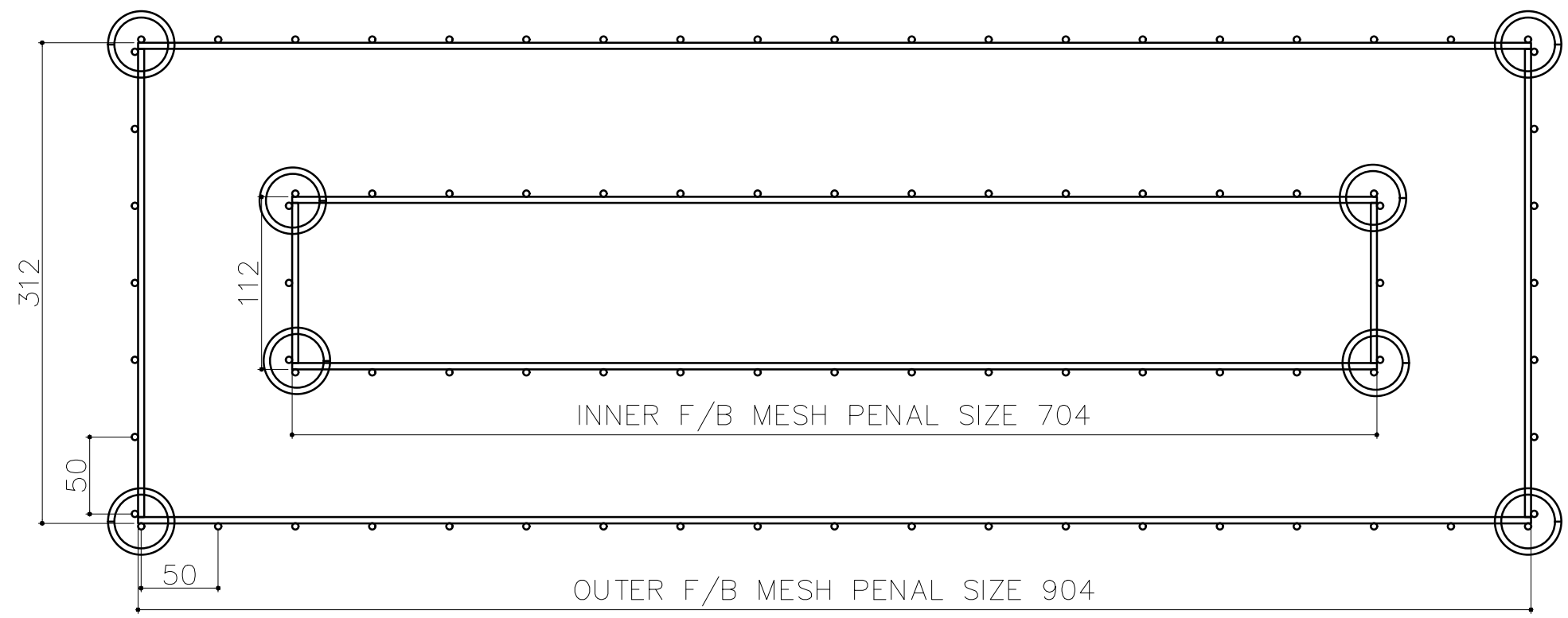
TOP / PLAN
