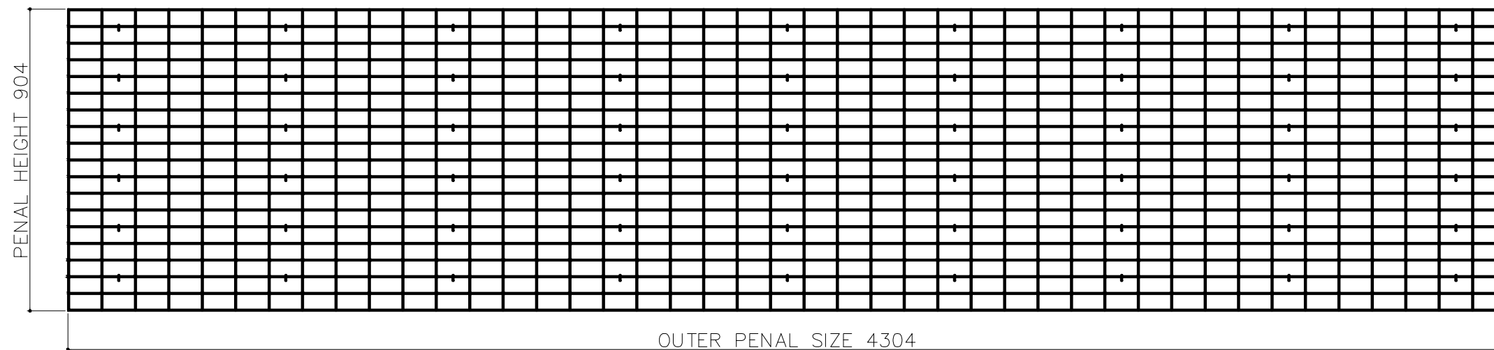
INNER FRONT BACK MESH PENAL QTY -02 (MESH WIRE Ø4MM) MESH SIZE 100X50
