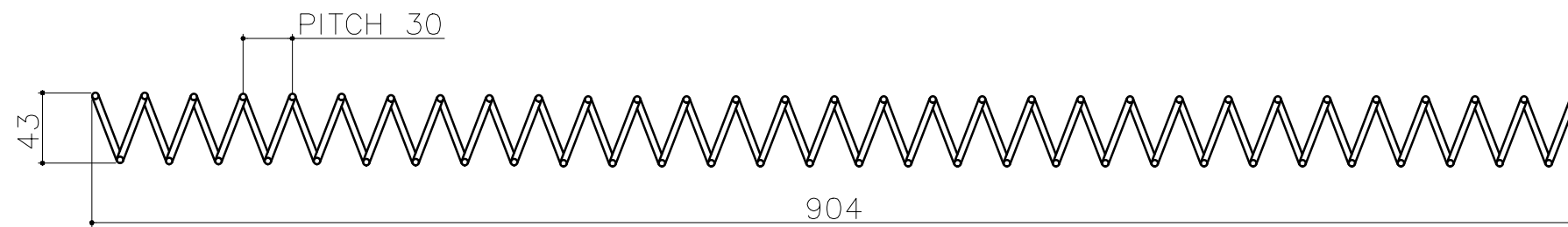
COIL WIRE Ø4MM ID-35 OD-43 NUMBER OF TURN 32 PITCH-30MM (QTY-08)
