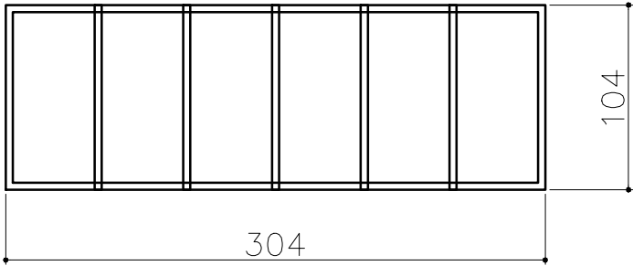
OUTER LEFT / RIGHT MESH PENAL MESH SIZE 100X50 (MESH WIRE DIA 4MM) QTY-02
