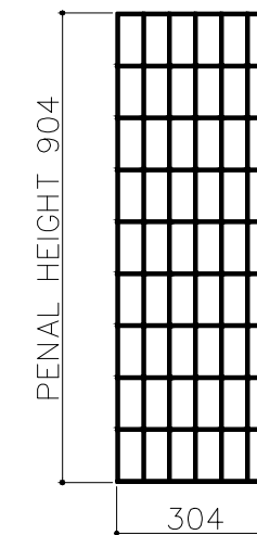
OUTER LEFT / RIGHT MESH PENAL QTY -02 (MESH WIRE Ø4MM) MESH SIZE 100X50
