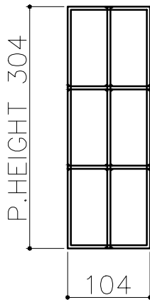
INNER LEFT RIGHT MESH PENAL QTY -02 (MESH WIRE Ø4MM)
