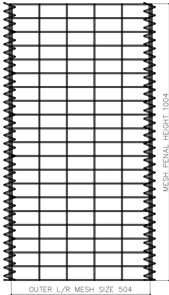
SIDE VIEW
