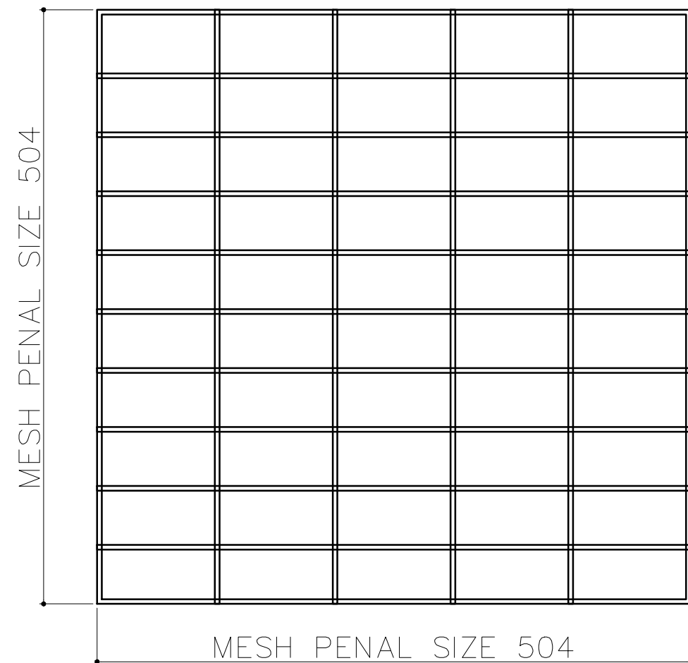
OUTER MESH PENAL QTY -04 (MESH WIRE Ø4MM) MESH SIZE 100X50
