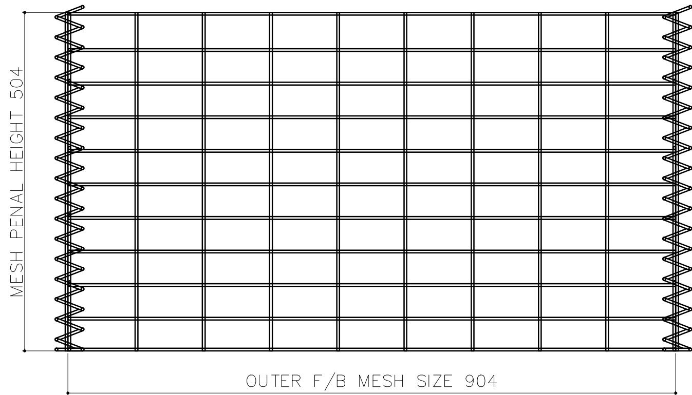
TYPICAL ELEVATION
