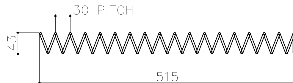
ID-35 OD-43 (COIL LENGTH -515) (COIL WIRE Ø4MM) (NUMBER OF TURN 18) (PITCH-30MM (QTY-05))
