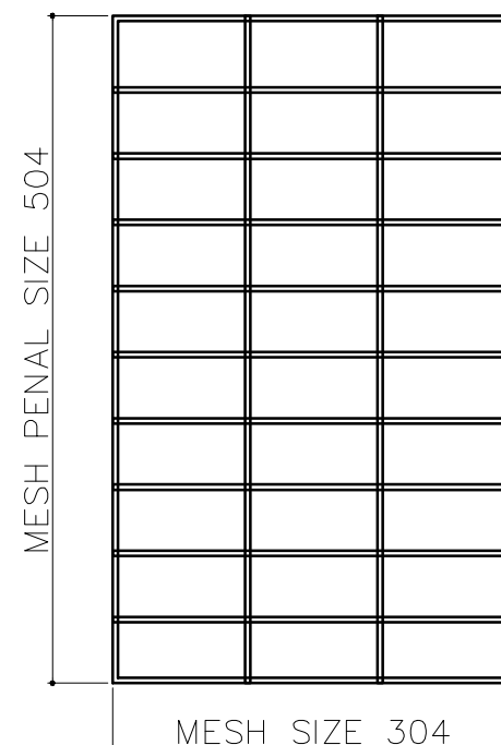
INNER L/R MESH PENAL QTY -02 (MESH WIRE Ø4MM) MESH SIZE 100X50
