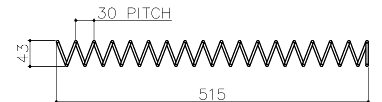
ID-35 OD-43 (COIL LENGTH -515) (COIL WIRE Ø4MM) (NUMBER OF TURN 18) (PITCH-30MM (QTY-05))
