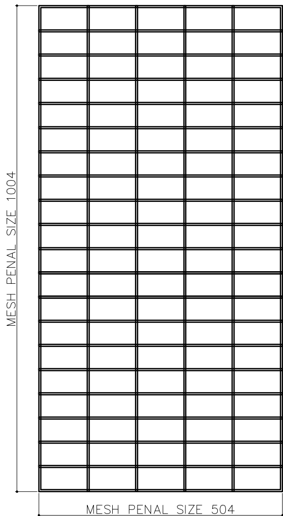
OUTER L/R MESH PENAL QTY -02 (MESH WIRE Ø4MM) MESH SIZE 100X50
