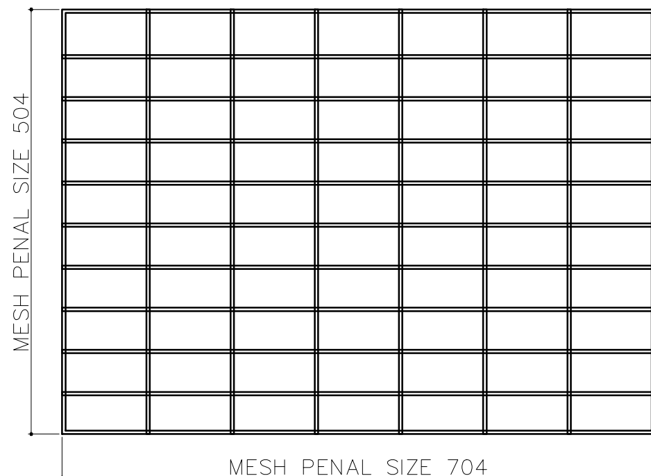
INNER F/B MESH PENAL QTY -02 (MESH WIRE Ø4MM) MESH SIZE 100X50
