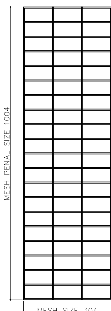
INNER L/R MESH PENAL QTY -02 (MESH WIRE Ø4MM) MESH SIZE 100X50
