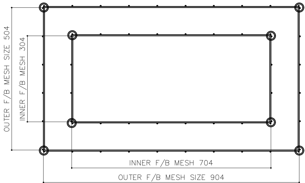
TOP / PLAN
