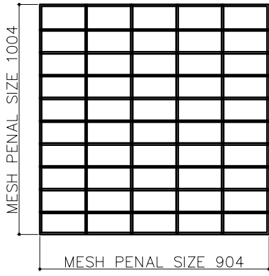
OUTER L/R MESH PENAL QTY -02 (MESH WIRE Ø4MM) MESH SIZE 100X50
