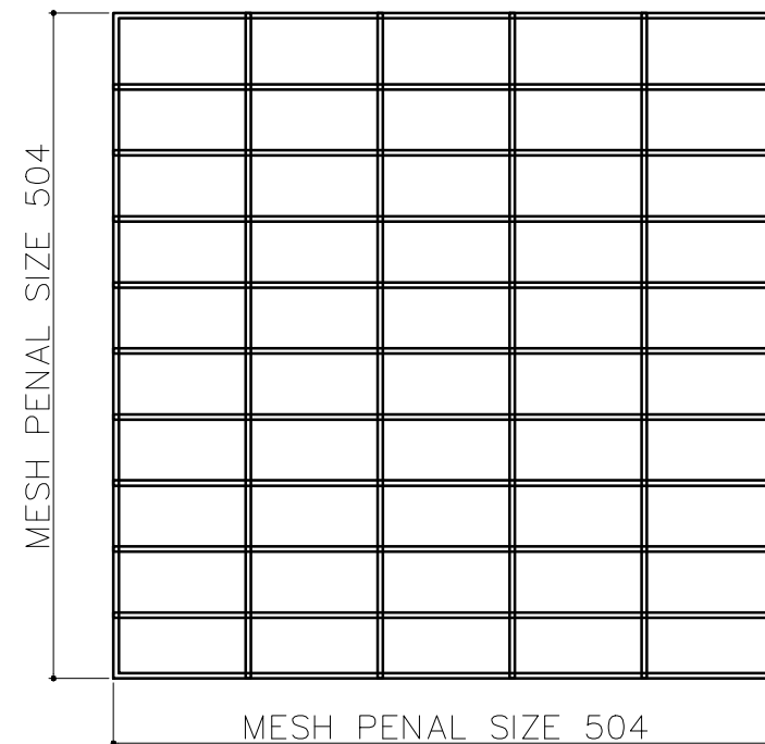
OUTER L/R MESH PENAL QTY -02 (MESH WIRE Ø4MM) MESH SIZE 100X50
