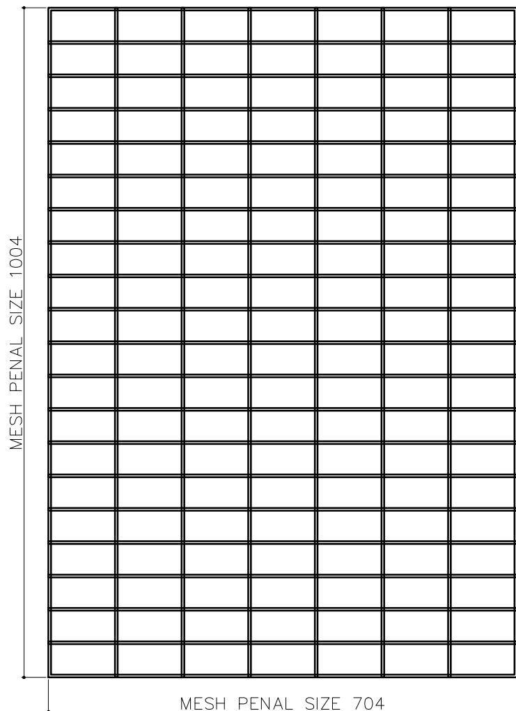
INNER F/B MESH PENAL QTY -02 (MESH WIRE Ø4MM) MESH SIZE 100X50
