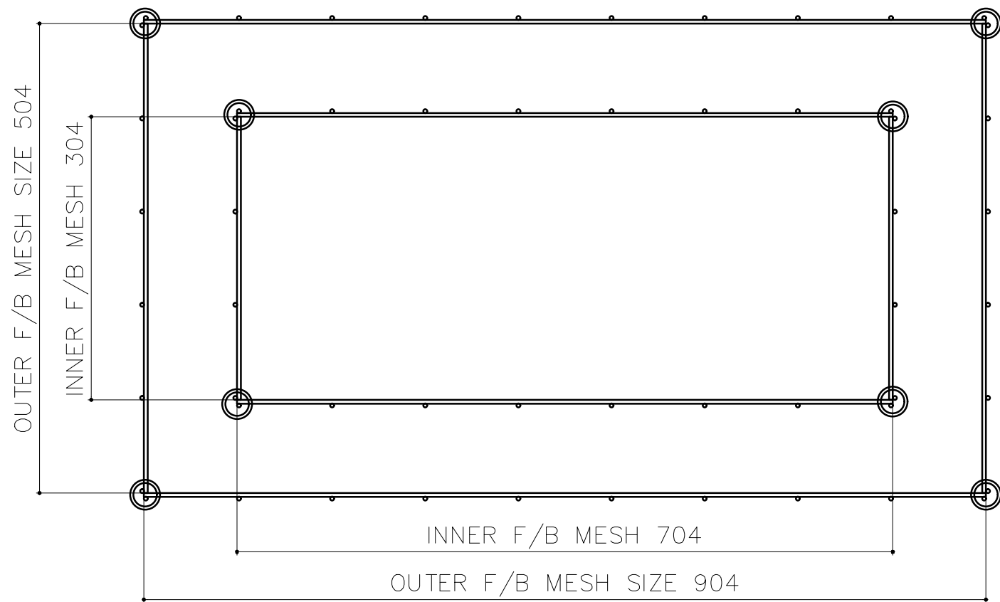
TOP / PLAN
