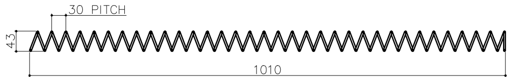
ID-35 OD-43 (COIL LENGTH -1010) (COIL WIRE Ø4MM) (NUMBER OF TURN 35) (PITCH-30MM (QTY-05))
