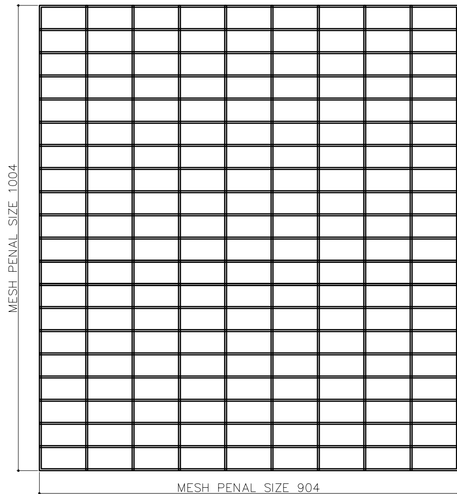
OUTER F/B MESH PENAL QTY -02 (MESH WIRE Ø4MM) MESH SIZE 100X50
