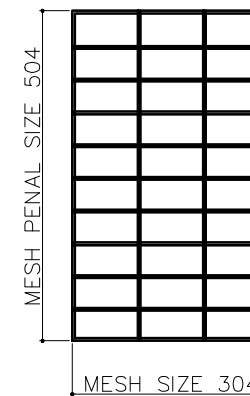
INNER L/R MESH PENAL QTY -02 (MESH WIRE Ø4MM) MESH SIZE 100X50
