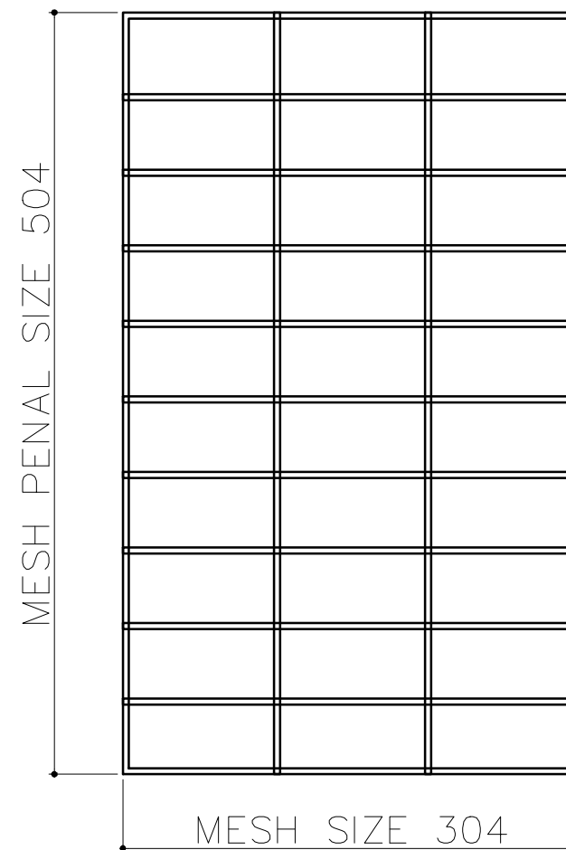
INNER MESH PENAL QTY -04 (MESH WIRE Ø4MM) MESH SIZE 100X50
