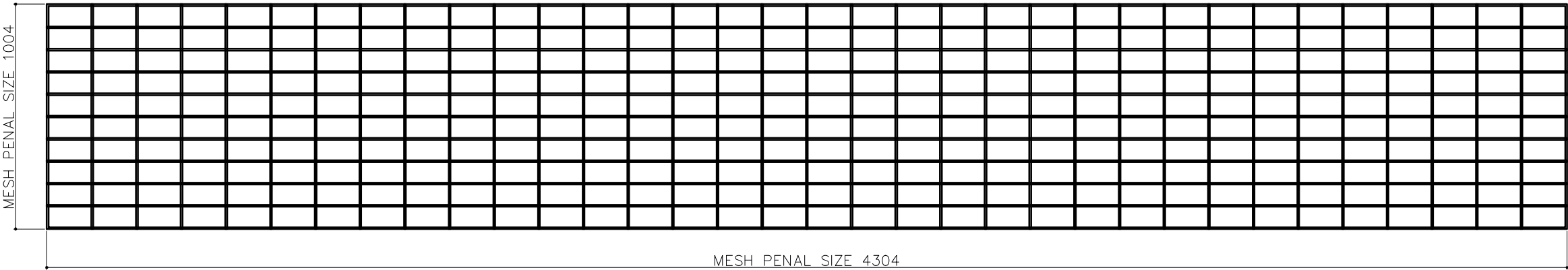
INNER F/B MESH PENAL QTY -02 (MESH WIRE Ø4MM) MESH SIZE 100X50
