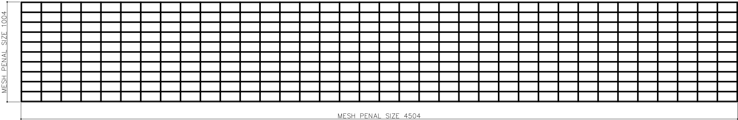
OUTER F/B MESH PENAL QTY -02 (MESH WIRE Ø4MM) MESH SIZE 100X50
