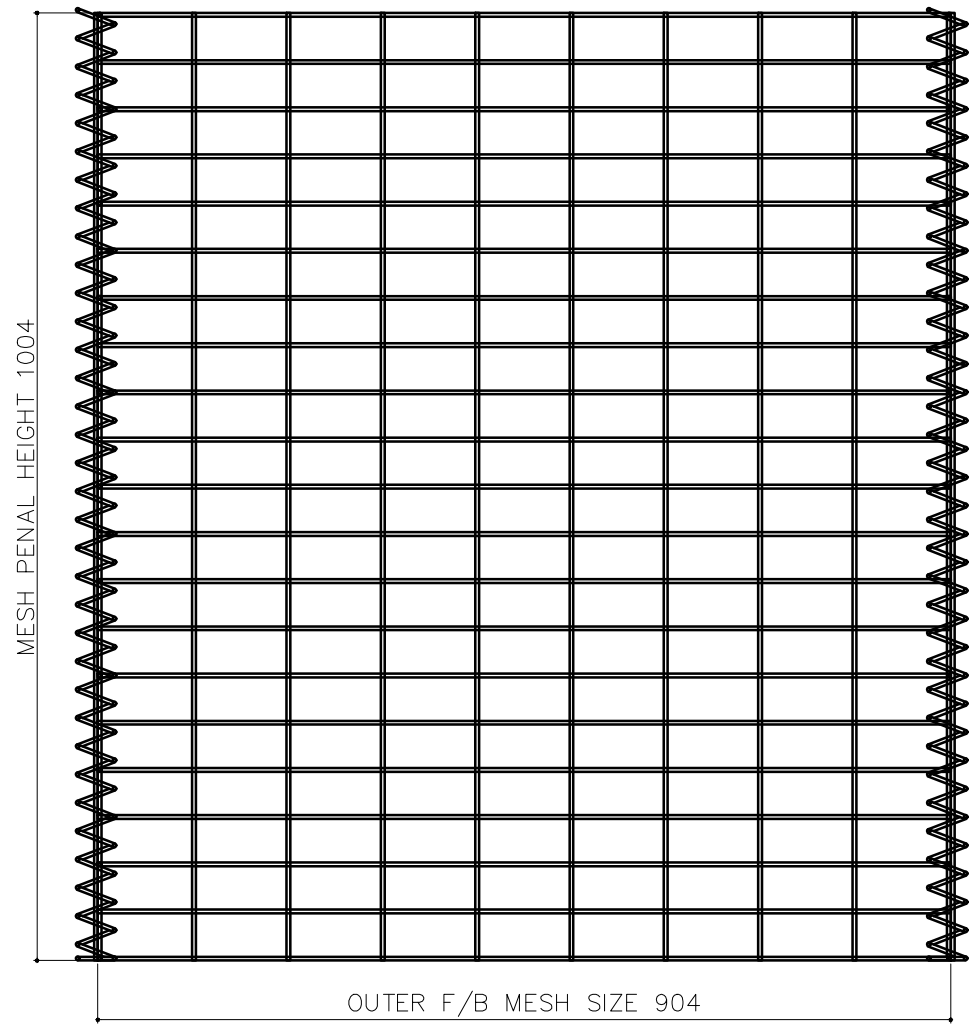
TYPICAL ELEVATION
