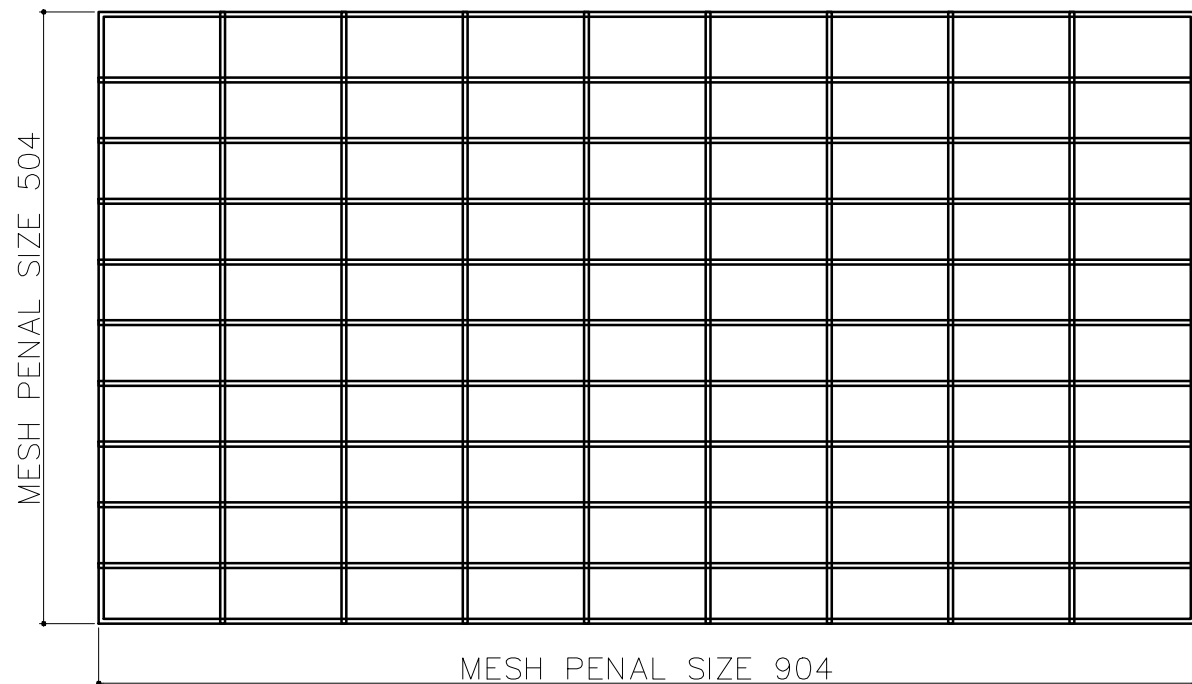
OUTER F/B MESH PENAL QTY -02 (MESH WIRE Ø4MM) MESH SIZE 100X50
