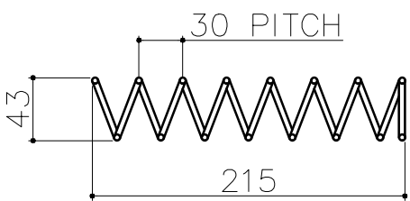
ID-35 OD-43 COIL LENGTH -215 COIL WIRE Ø4MM NUMBER OF TURN 09 PITCH-30MM (QTY-08)
