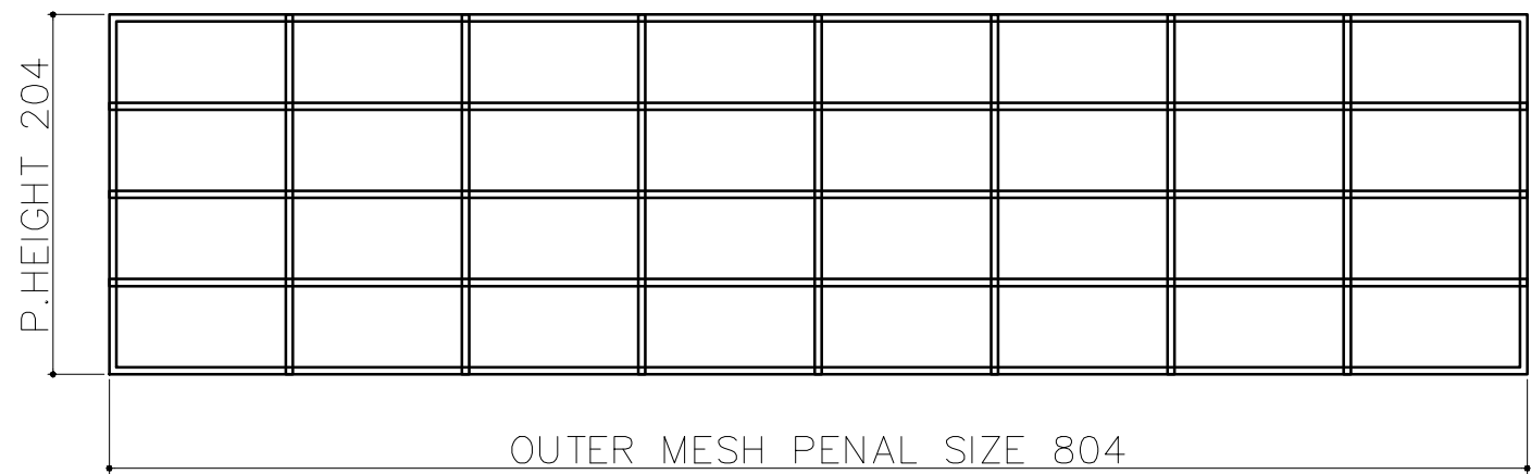
INNER FRONT BACK LEFT RIGHT MESH PENAL QTY -04 MESH WIRE Ø4MM) MESH SIZE 100X50
