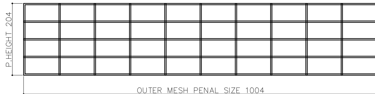
OUTER LEFT RIGHT MESH PENAL QTY -02 MESH WIRE Ø4MM) MESH SIZE 100X50
