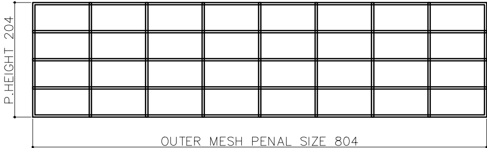
INNER FRONT BACK LEFT RIGHT MESH PENAL QTY -02 MESH WIRE Ø4MM) MESH SIZE 100X50
