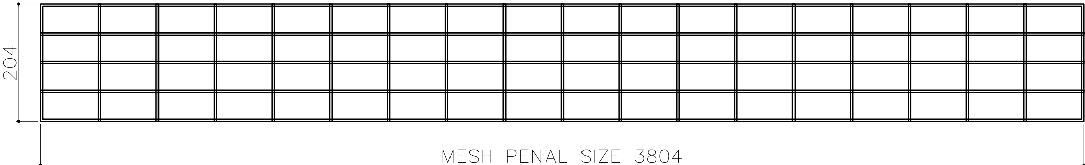
INNER FRONT BACK MESH PENAL QTY -02 MESH WIRE Ø4MM) MESH SIZE 100X50
