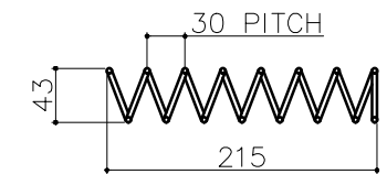
ID-35 OD-43 COIL LENGTH -215 COIL WIRE Ø4MM NUMBER OF TURN 09 PITCH-30MM (QTY-08)
