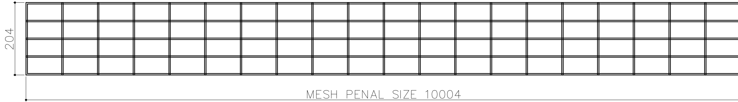
OUTER FRONT BACK MESH PENAL QTY -02 MESH WIRE Ø4MM) MESH SIZE 100X50
