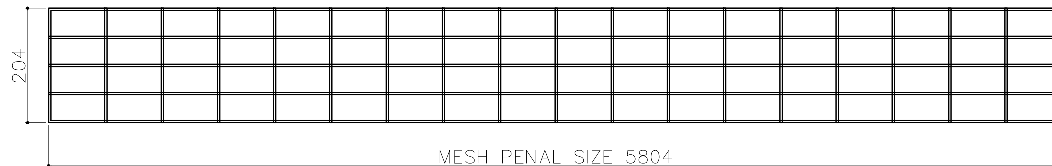
INNER FRONT BACK MESH PENAL QTY -02 MESH WIRE Ø4MM) MESH SIZE 100X50
