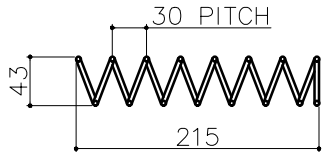
ID-35 OD-43 COIL LENGTH -215 COIL WIRE Ø4MM NUMBER OF TURN 09 PITCH-30MM (QTY-08)
