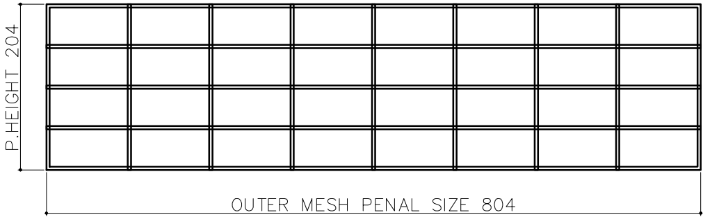
INNER FRONT BACK LEFT RIGHT MESH PENAL QTY -02 MESH WIRE Ø4MM) MESH SIZE 100X50
