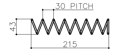
ID-35 OD-43 COIL LENGTH -215 COIL WIRE Ø4MM NUMBER OF TURN 09 PITCH-30MM (QTY-08)
