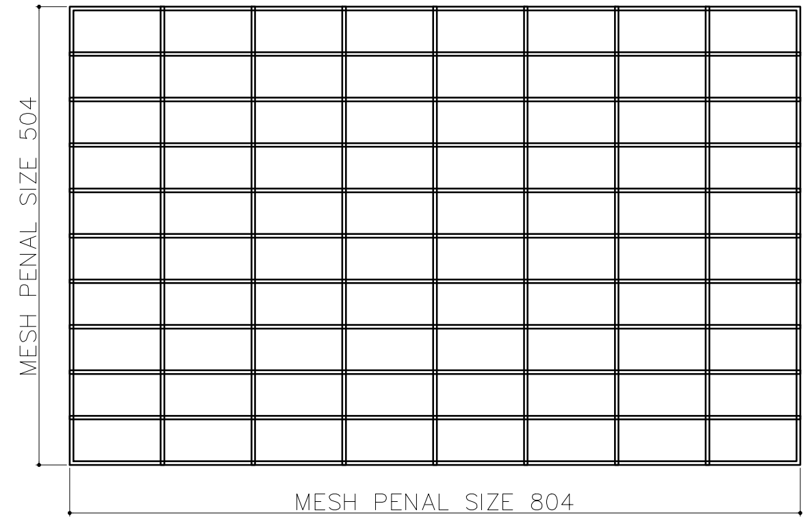
INNER MESH PENAL QTY -01 (MESH WIRE Ø4MM) MESH SIZE 100X50
