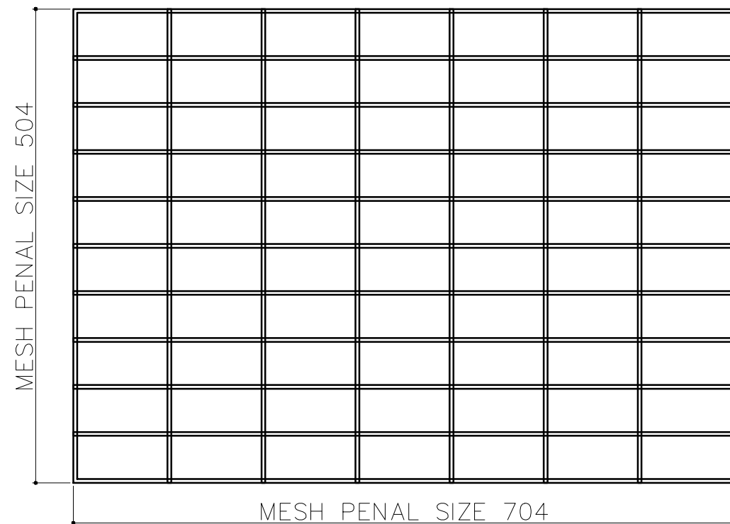
LEFT / RIGHT MESH PENAL QTY -02 (MESH WIRE Ø4MM) MESH SIZE 100X50
