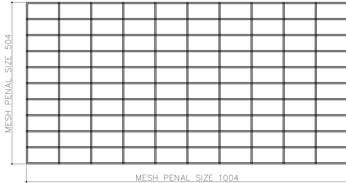
FRONT MESH PENAL QTY -01 (MESH WIRE Ø4MM) MESH SIZE 100X50
