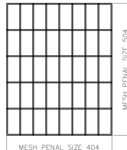
INNER HEX MESH PENAL QTY -06 (MESH WIRE Ø4MM) MESH SIZE 100X50
