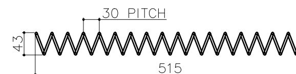
ID-35 OD-43 COIL LENGTH -1010 COIL WIRE Ø4MM NUMBER OF TURN 18 PITCH-30MM (QTY-12)
