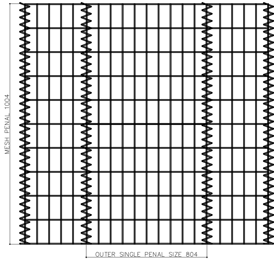
TYPICAL ELEVATION
