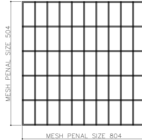
OUTER HEX MESH PENAL QTY -06 (MESH WIRE Ø4MM) MESH SIZE 100X50
