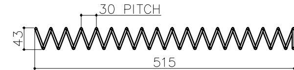
ID-35 OD-43 COIL LENGTH -1010 COIL WIRE Ø4MM NUMBER OF TURN 18 PITCH-30MM (QTY-12)
