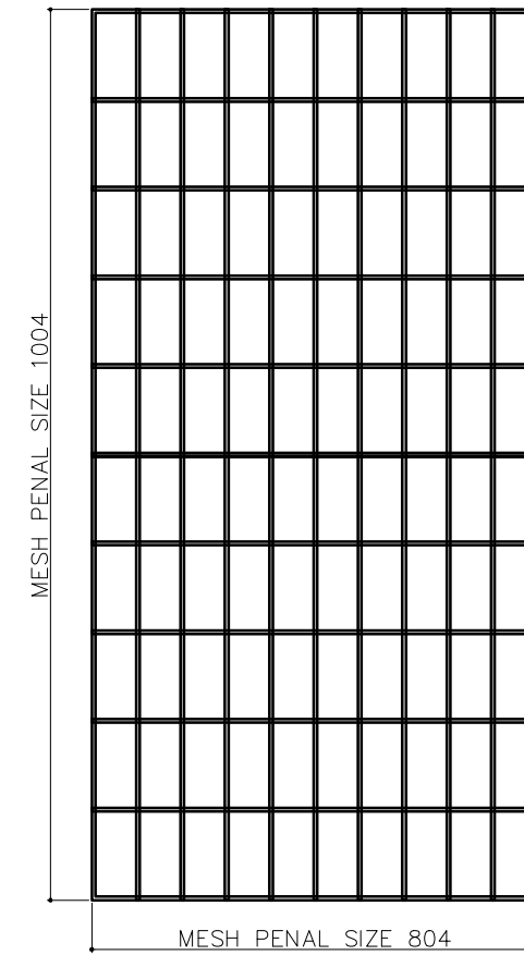
OUTER HEX MESH PENAL QTY -06 (MESH WIRE Ø4MM) MESH SIZE 100X50
