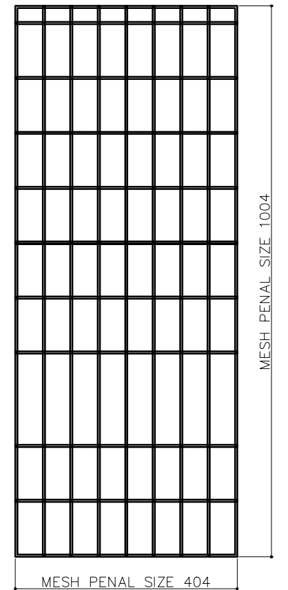
INNER HEX MESH PENAL QTY -06 (MESH WIRE Ø4MM) MESH SIZE 100X50
