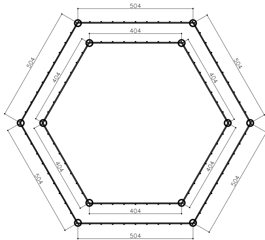
TOP / PLAN
