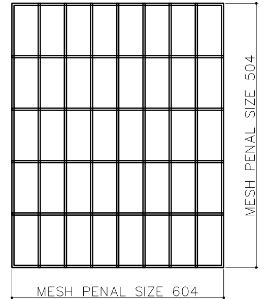
INNER HEX MESH PENAL QTY -06 (MESH WIRE Ø4MM) MESH SIZE 100X50
