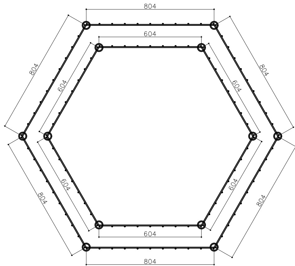
TOP / PLAN
