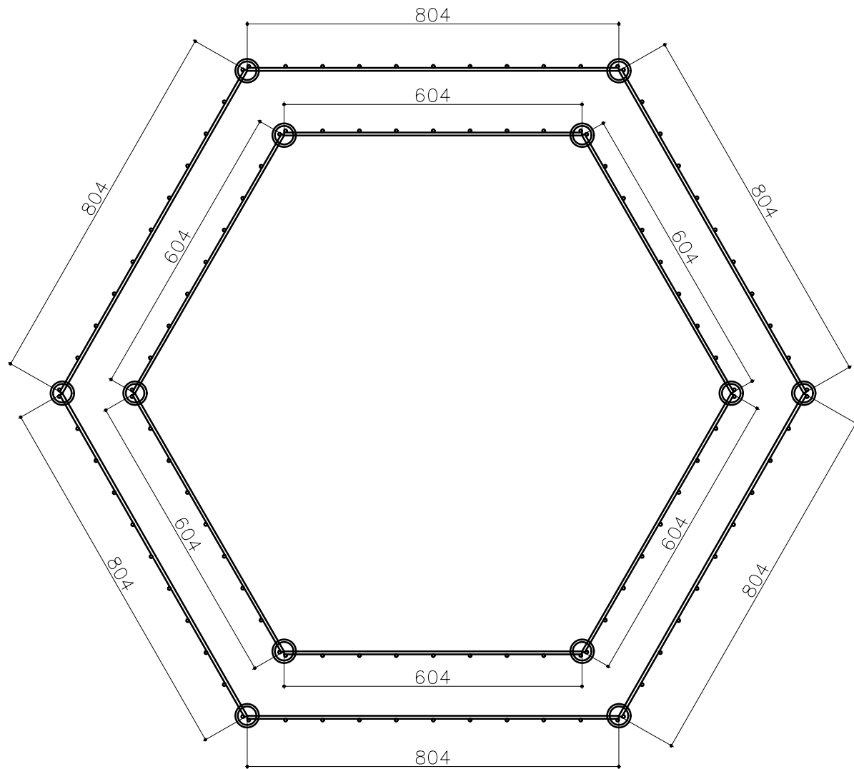
TOP / PLAN
