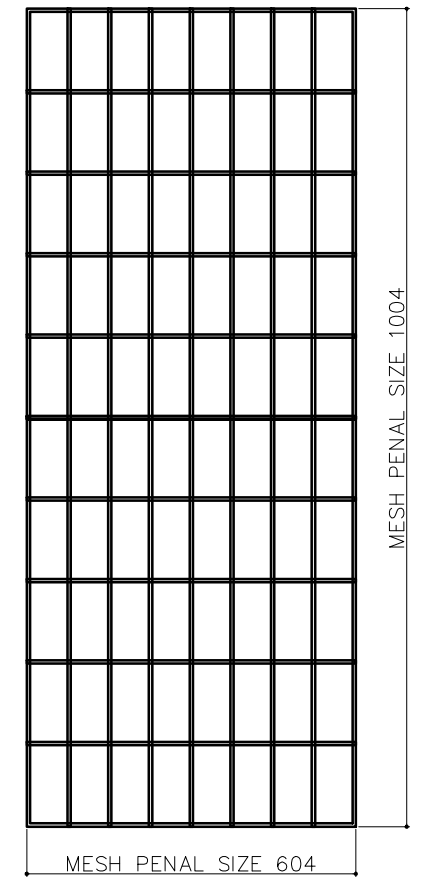
INNER HEX MESH PENAL QTY -06 (MESH WIRE Ø4MM) MESH SIZE 100X50
