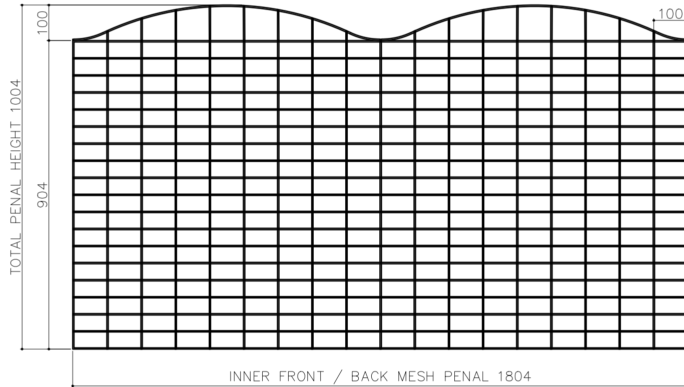
INNER FRONT BACK MESH PENAL QTY-02 (MESH SIZE - 50X100) WIRE DIA 4MM
