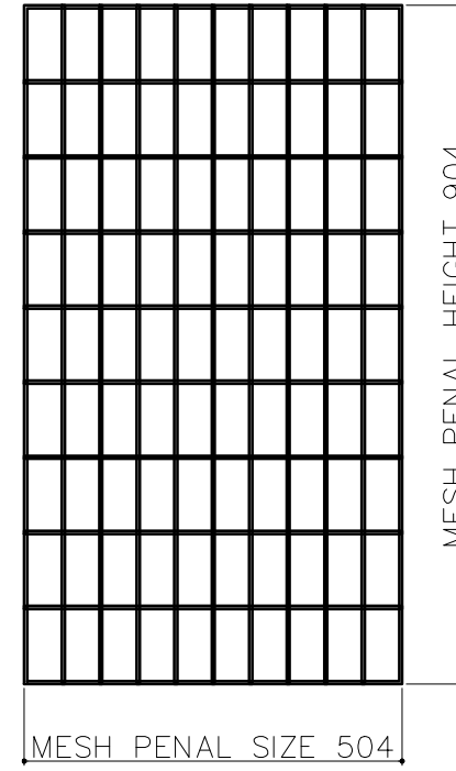
OUTER L/R MESH PENAL QTY-02 (MESH SIZE - 50X100) WIRE DIA 4MM
