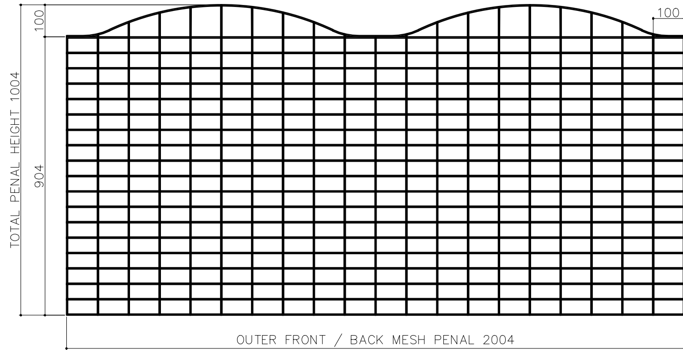
OUTER FRONT BACK MESH PENAL QTY-02 (MESH SIZE - 50X100) WIRE DIA 4MM
