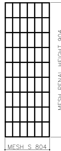
INNER L/R MESH PENAL QTY-02 (MESH SIZE - 50X100) WIRE DIA 4MM
