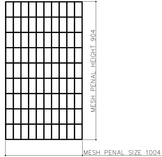
OUTER L/R MESH PENAL QTY-02 (MESH SIZE - 50X100) WIRE DIA 4MM
