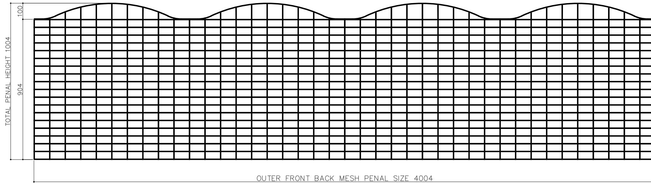
OUTER FRONT BACK MESH PENAL QTY-02 (MESH SIZE - 50X100) WIRE DIA 4MM
