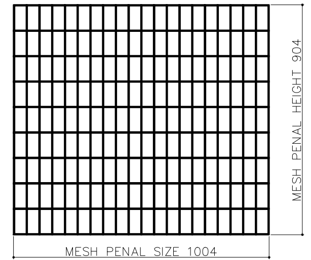
OUTER L/R MESH PENAL QTY-02 (MESH SIZE - 50X100) WIRE DIA 4MM
