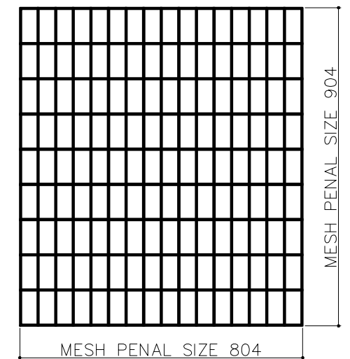
INNER L/R MESH PENAL QTY-02 (MESH SIZE - 50X100) WIRE DIA 4MM
