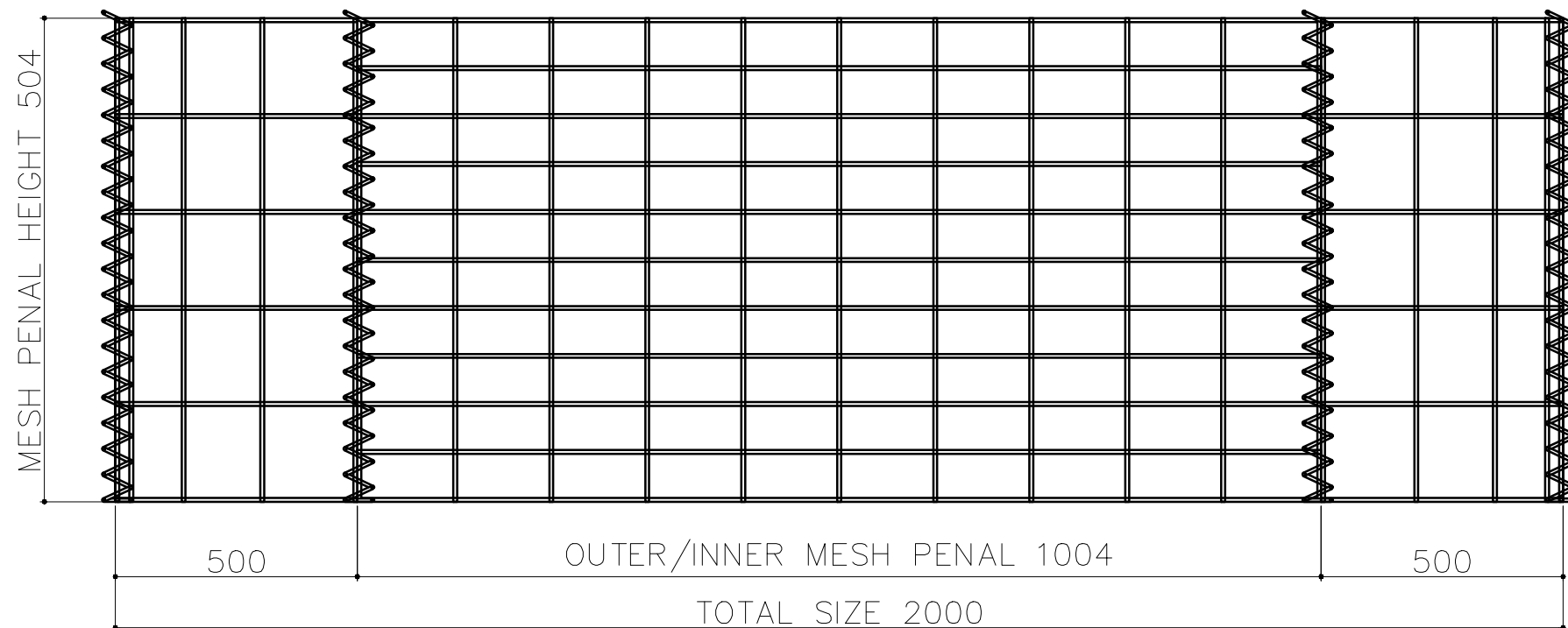
TYPICAL ELEVATION
