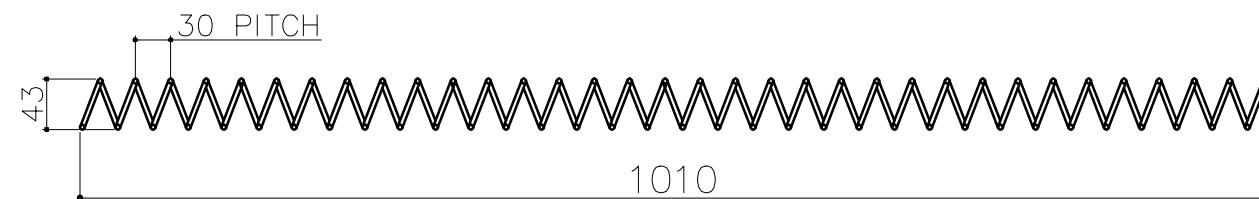
ID-35 OD-43 COIL LENGTH - 1010 COIL WIRE Ø4MM NUMBER OF TURN 36 PITCH-30MM (QTY-08)
