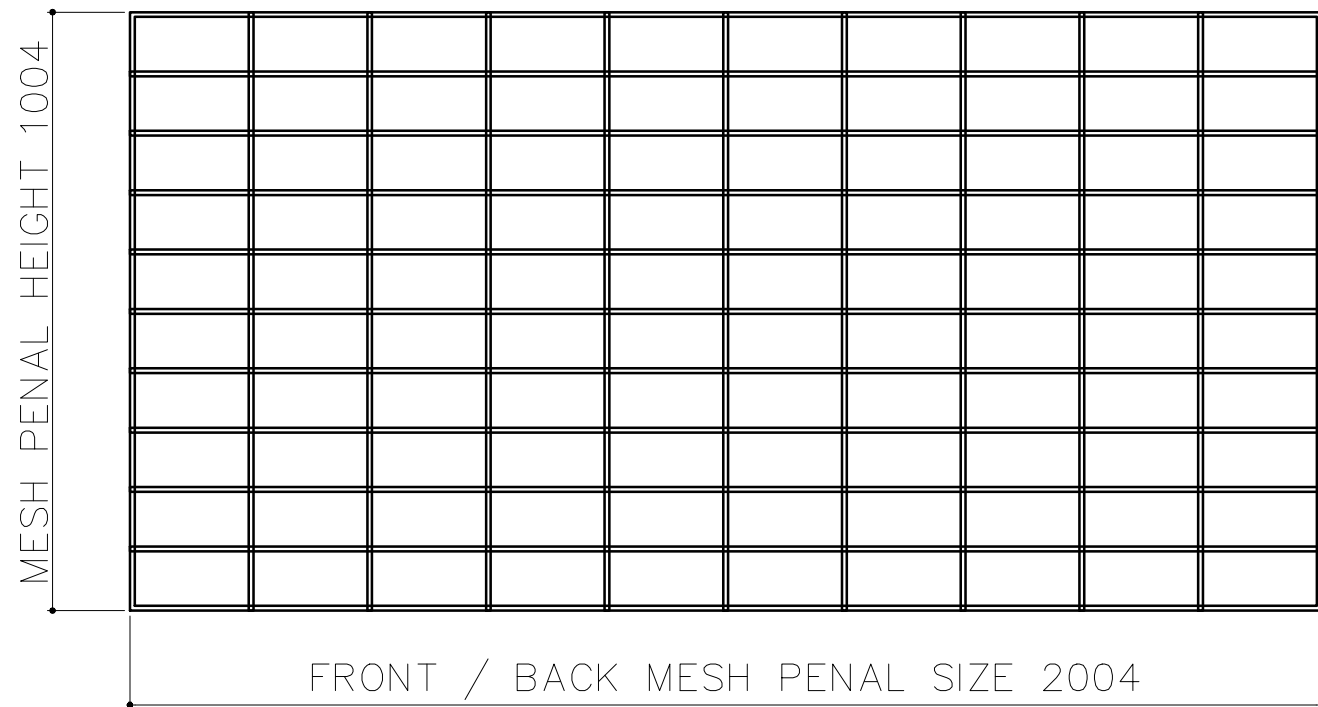
OUTER INNER FRONT BACK MESH PENAL QTY-04 (MESH SIZE - 50X100)
