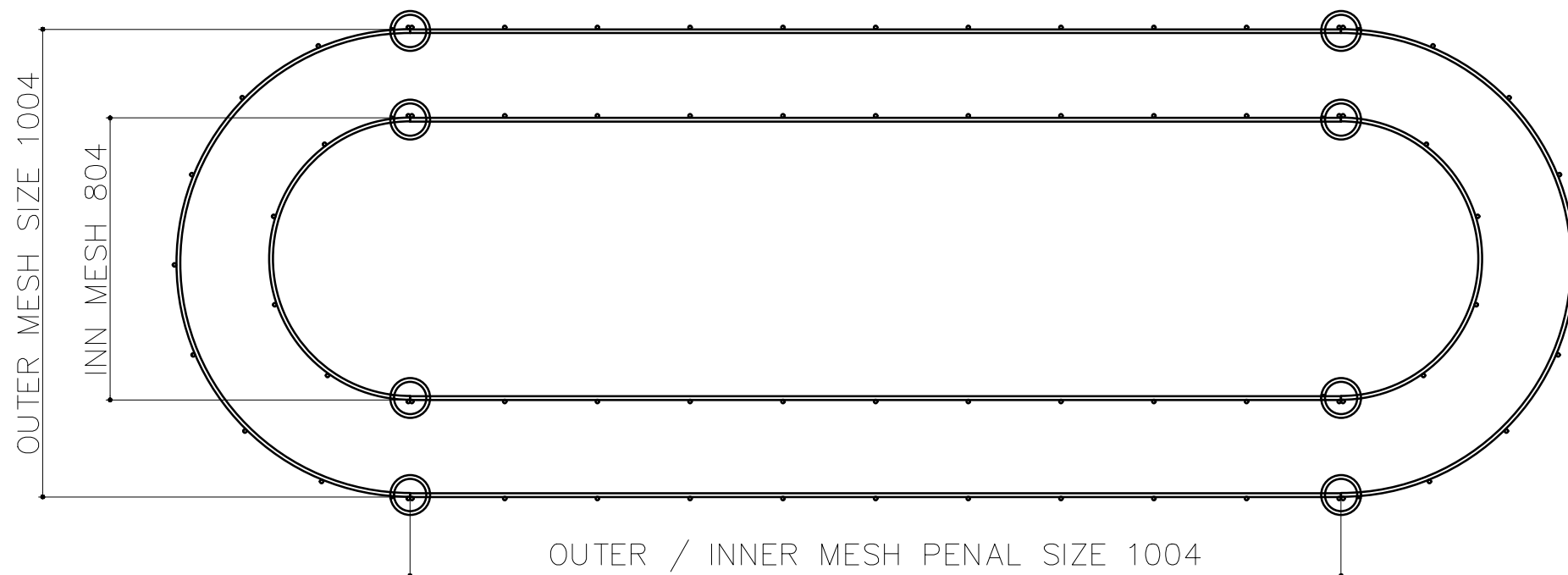
PLAN / TOP
