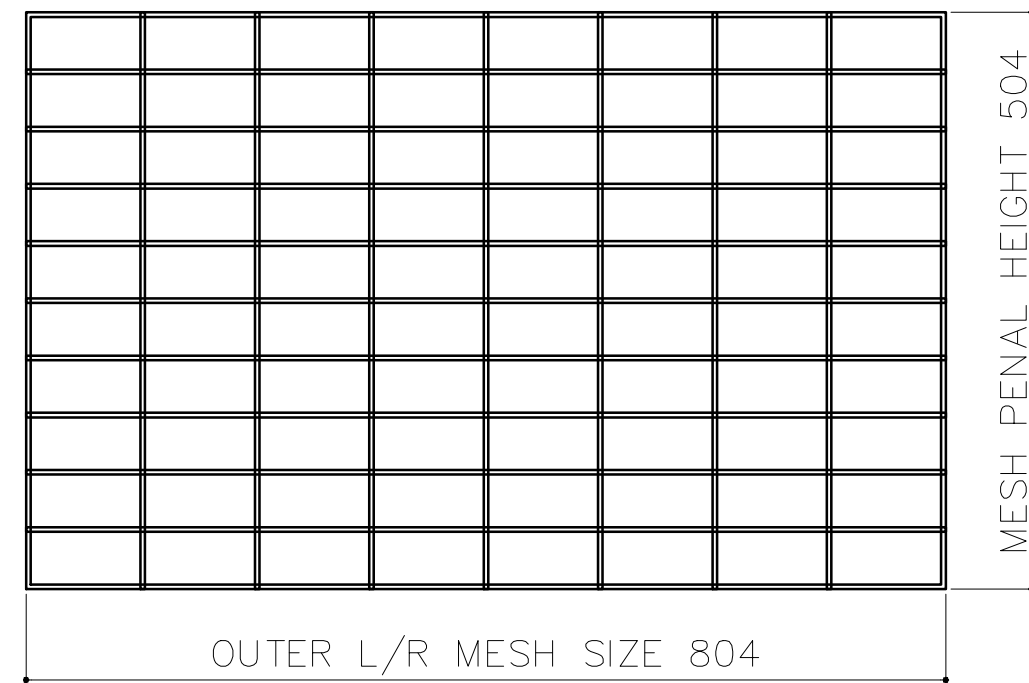
OUTER L/R MESH PENAL QTY-02 (MESH SIZE - 50X100)
