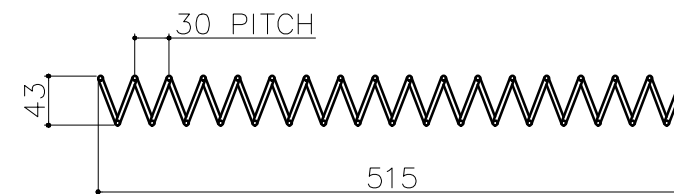
ID-35 OD-43 COIL LENGTH -515 COIL WIRE Ø4MM NUMBER OF TURN 18 PITCH-30MM (QTY-08)
