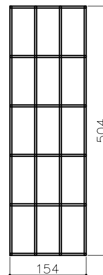
CENTER POST TOP BOTTOM MESH PENAL QTY -02 (MESH WIRE Ø4MM) MESH SIZE 100X50
