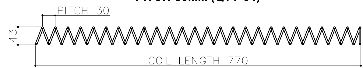
ID-35 OD-43 COIL LENGTH -770 COIL WIRE Ø4MM NUMBER OF TURN 28 PITCH-30MM (QTY-04)
