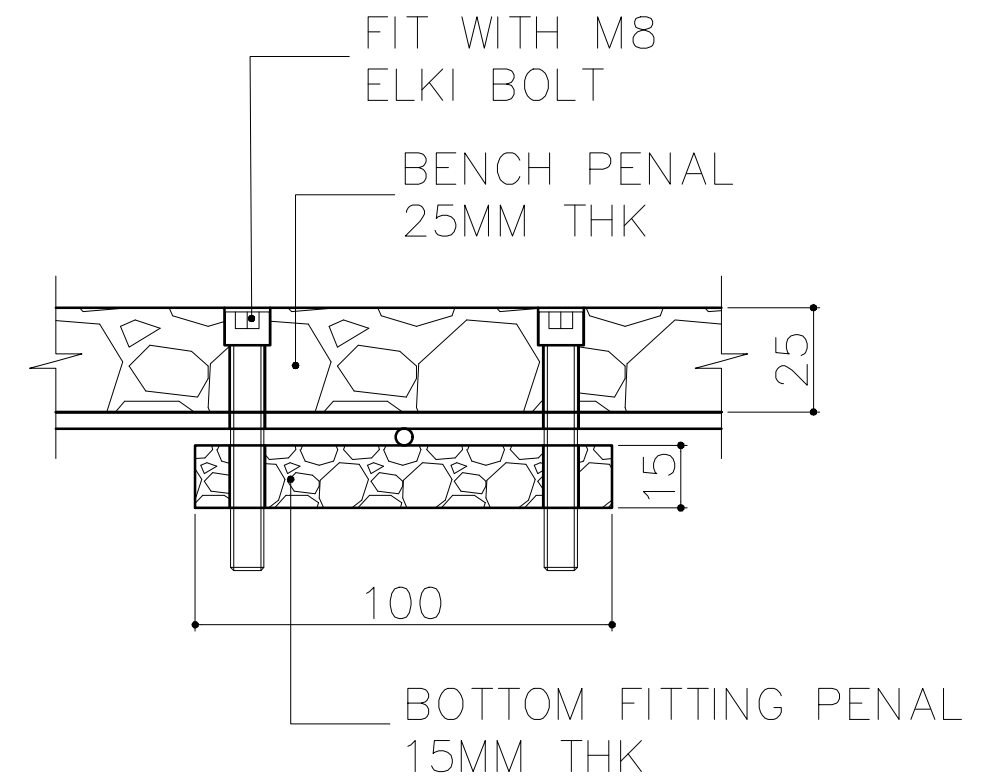
DETAIL "B"
