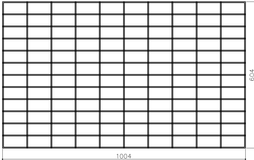
BENCH TOP/BOTTOM MESH PENAL QTY -04 (MESH WIRE Ø4MM) MESH SIZE 100X50
