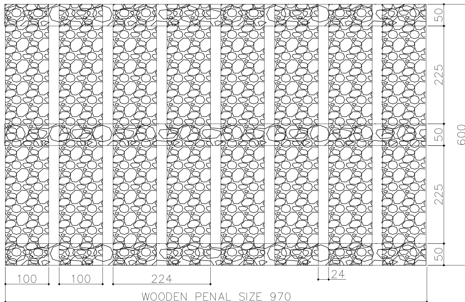
BOTTOM WOODEN PENAL (QTY-01)
