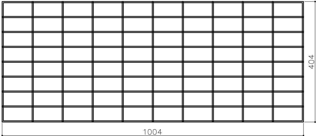
BENCH FRONT MESH PENAL QTY -02 (MESH WIRE Ø4MM) MESH SIZE 100X50
