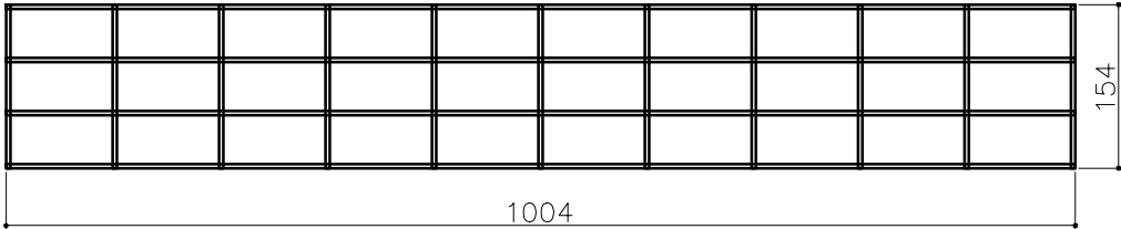
BACK TOP BOTTOM MESH PENAL QTY -04 (MESH WIRE Ø4MM) MESH SIZE 100X50
