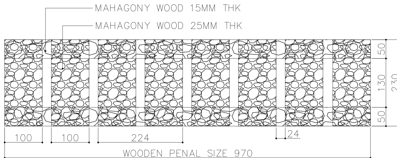
TOP WOODEN PENAL (QTY-01)
