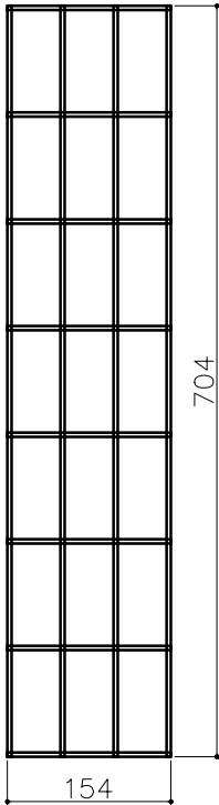
BACK SIDE MESH PENAL QTY -04 (MESH WIRE Ø4MM) MESH SIZE 100X50
