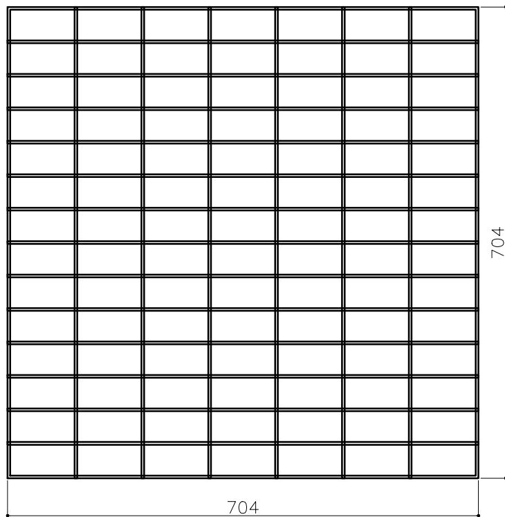
CENTER POST OUTER FRONT / BACK MESH PENAL QTY -02 (MESH WIRE Ø4MM) MESH SIZE 100X50
