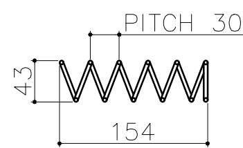
ID-35 OD-43 COIL LENGTH-154 COIL WIRE Ø4MM NUMBER OF TURN 06 PITCH-30MM (QTY-04)
