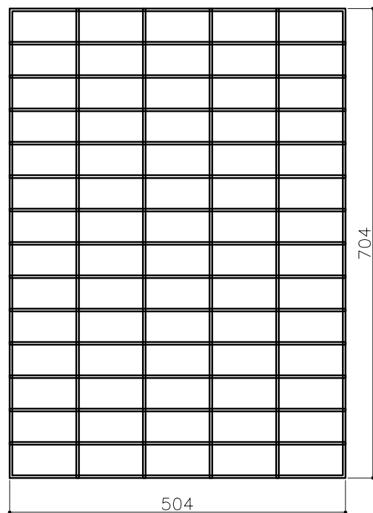
CENTER POST INNER FRONT / BACK MESH PENAL QTY -02 (MESH WIRE Ø4MM) MESH SIZE 100X50
