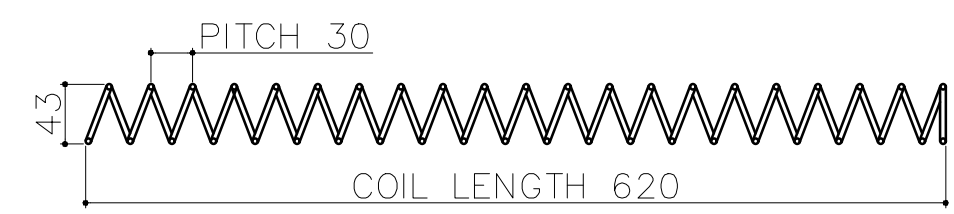
ID-35 OD-43 COIL LENGTH -620 COIL WIRE Ø4MM NUMBER OF TURN 22 PITCH-30MM (QTY-08)
