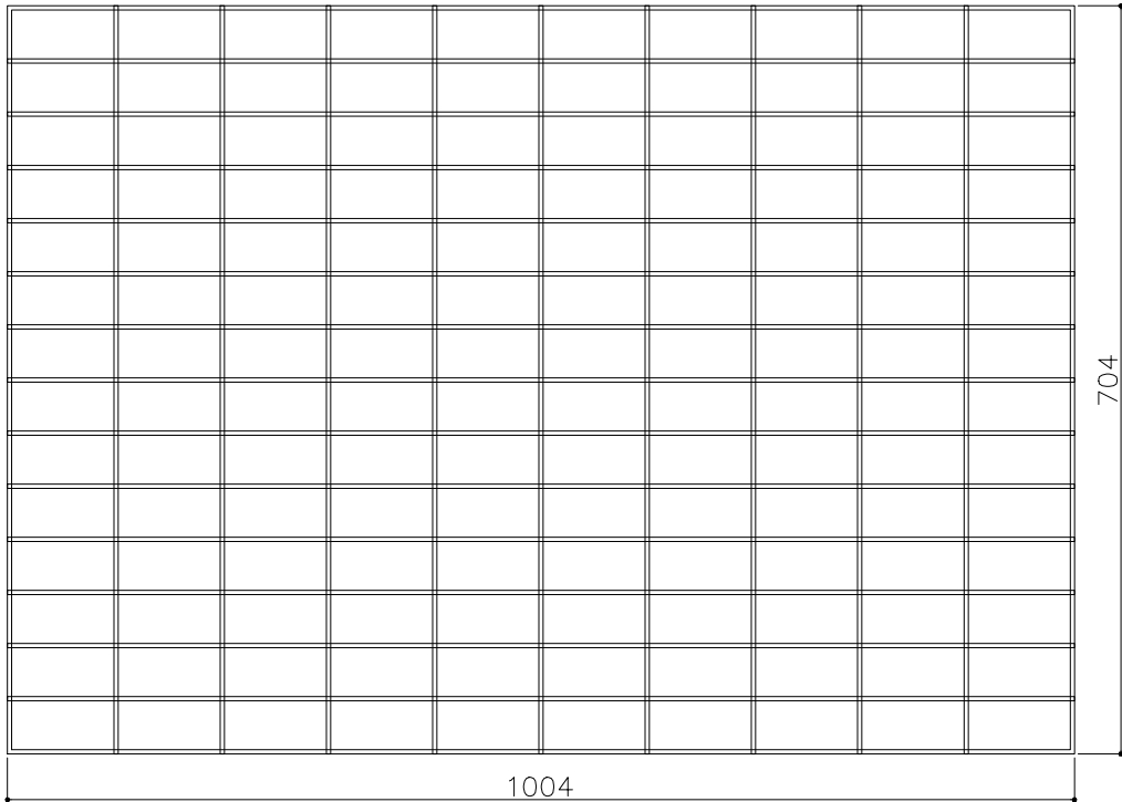
BACK MESH PENAL QTY -04 (MESH WIRE Ø4MM) MESH SIZE 100X50
