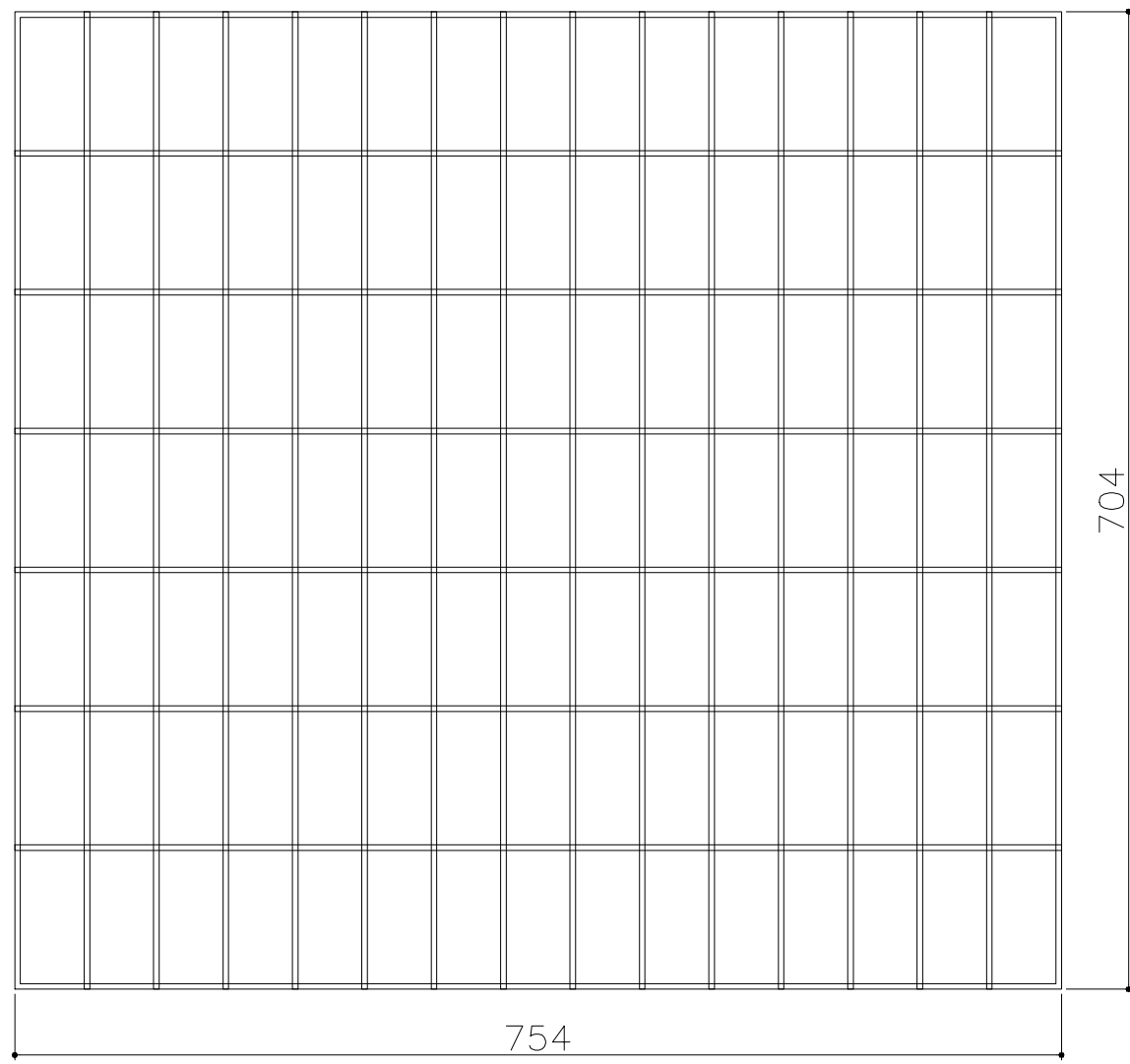
SIDE POSTS L/ R MESH PENAL QTY -04 (MESH WIRE Ø4MM) MESH SIZE 100X50
