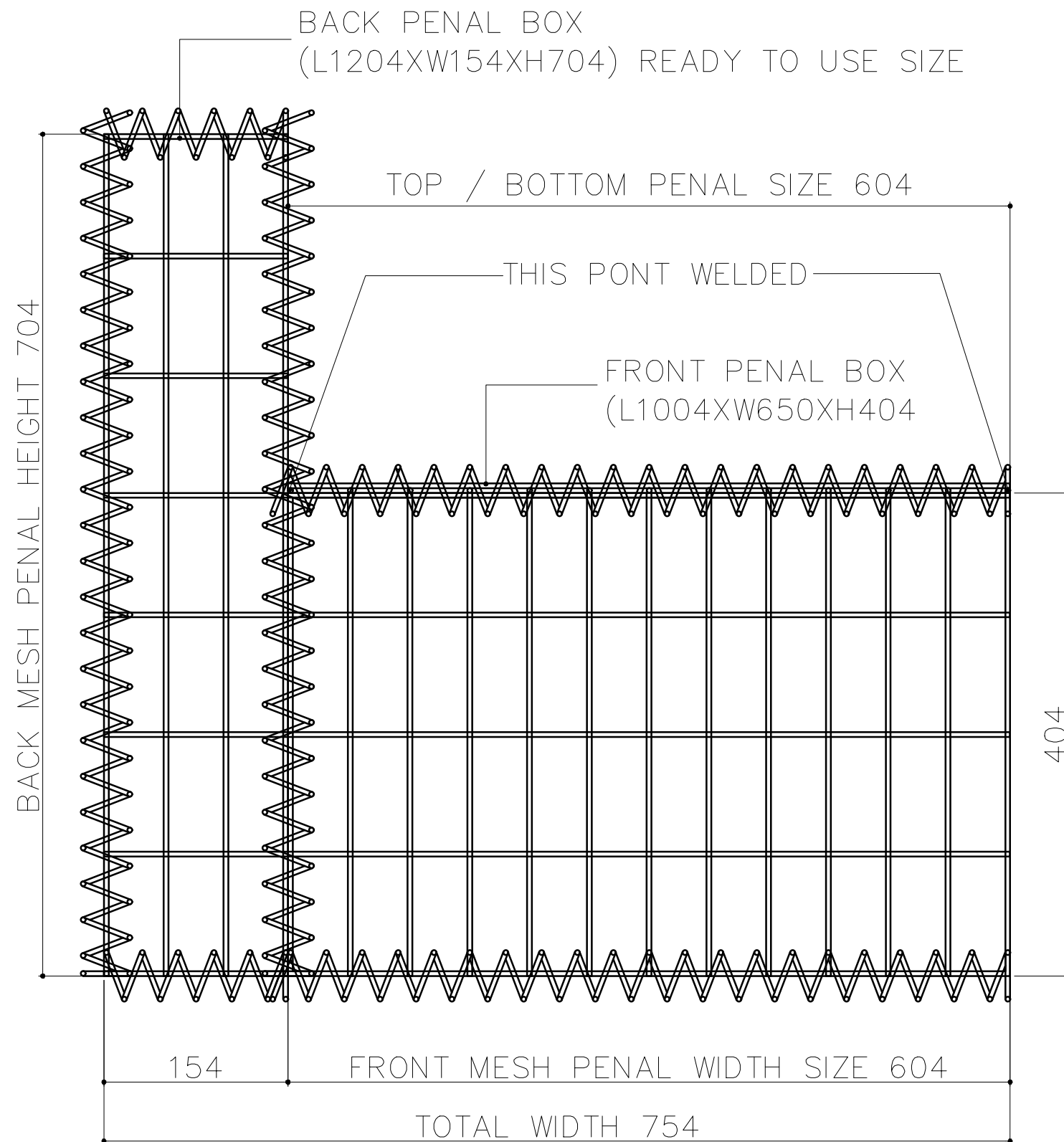
SECTION "A"
