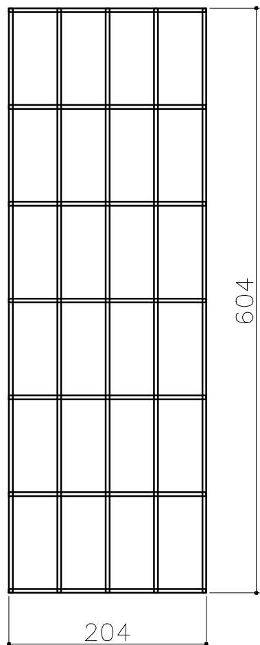
SIDE POSTS T/ B MESH PENAL QTY -04 (MESH WIRE Ø4MM) MESH SIZE 100X50
