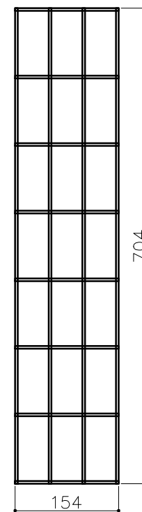
CENTER POST TOP BOTTOM MESH PENAL QTY -02 (MESH WIRE Ø4MM) MESH SIZE 100X50
