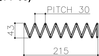
ID-35 OD-43 COIL LENGTH - 215 COIL WIRE Ø4MM NUMBER OF TURN 09 PITCH-30MM (QTY-08)
