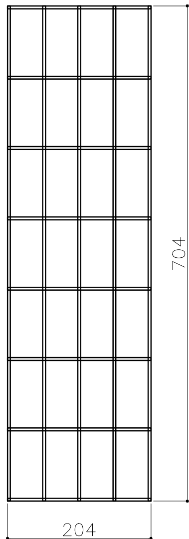
SIDE POSTS L/ R MESH PENAL QTY -04 (MESH WIRE Ø4MM) MESH SIZE 100X50
