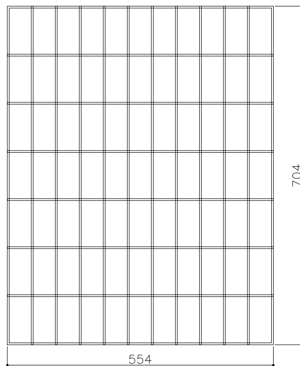
CENTER POST INNER L / R MESH PENAL QTY -02 (MESH WIRE Ø4MM) MESH SIZE 100X50
