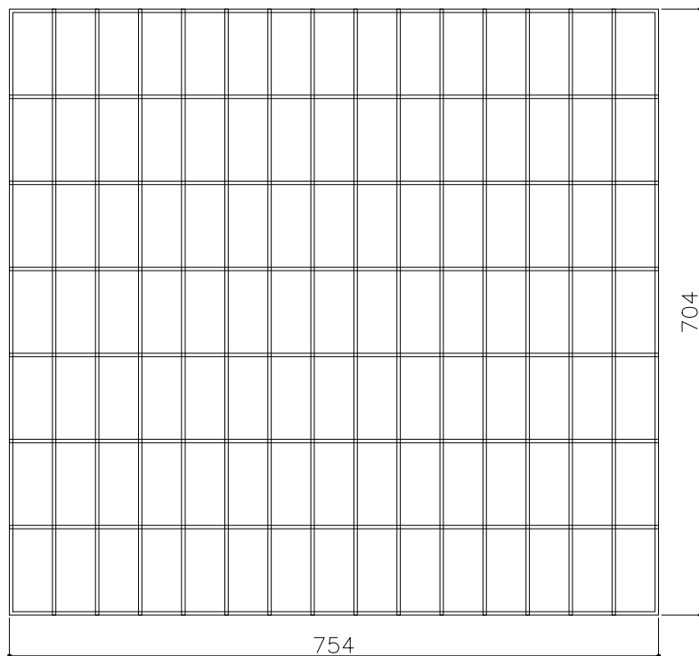
CENTER POST OUTER L / R MESH PENAL QTY -02 (MESH WIRE Ø4MM) MESH SIZE 100X50
