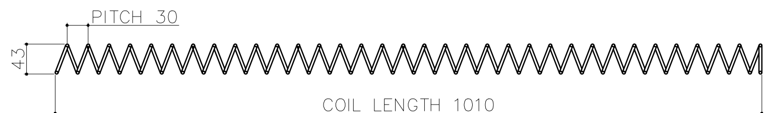
ID-35 OD-43 COIL LENGTH -1010 COIL WIRE Ø4MM NUMBER OF TURN 35 PITCH-30MM (QTY-08)
