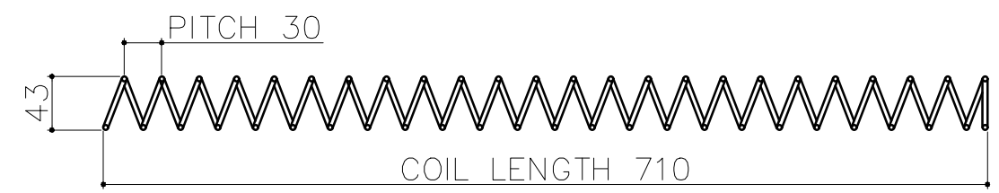
ID-35 OD-43 COIL LENGTH -710 COIL WIRE Ø4MM NUMBER OF TURN 26 PITCH-30MM (QTY-04)
