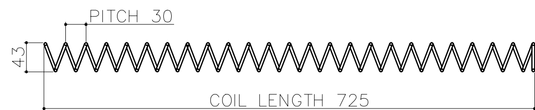
ID-35 OD-43 COIL LENGTH -725 COIL WIRE Ø4MM NUMBER OF TURN 26 PITCH-30MM (QTY-20)
