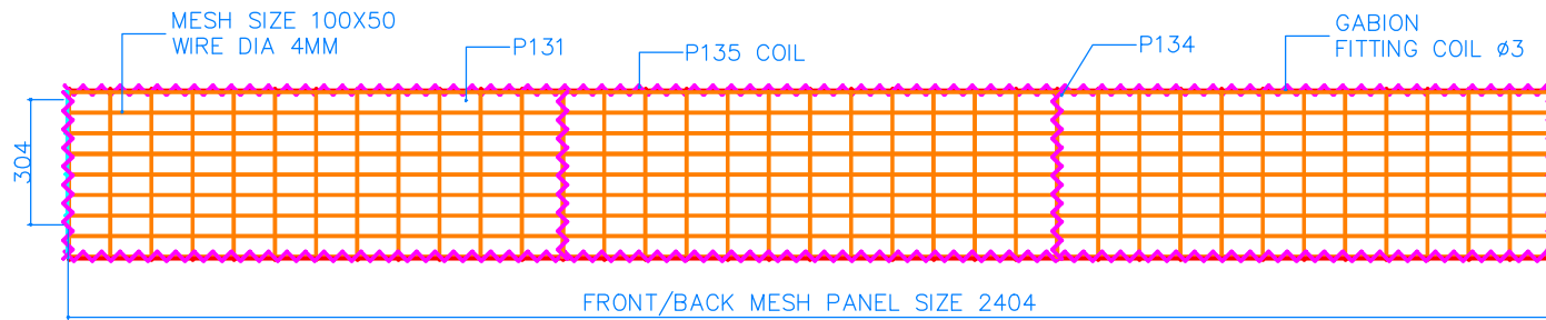
ELEVATION FRONT
