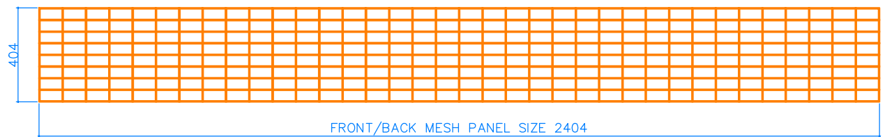
P131 FRONT/BACK MESH PANEL QTY-02 MESH SIZE 100X50 WIRE DIA 4MM
