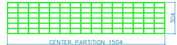
CENTER PARTITION 1504
