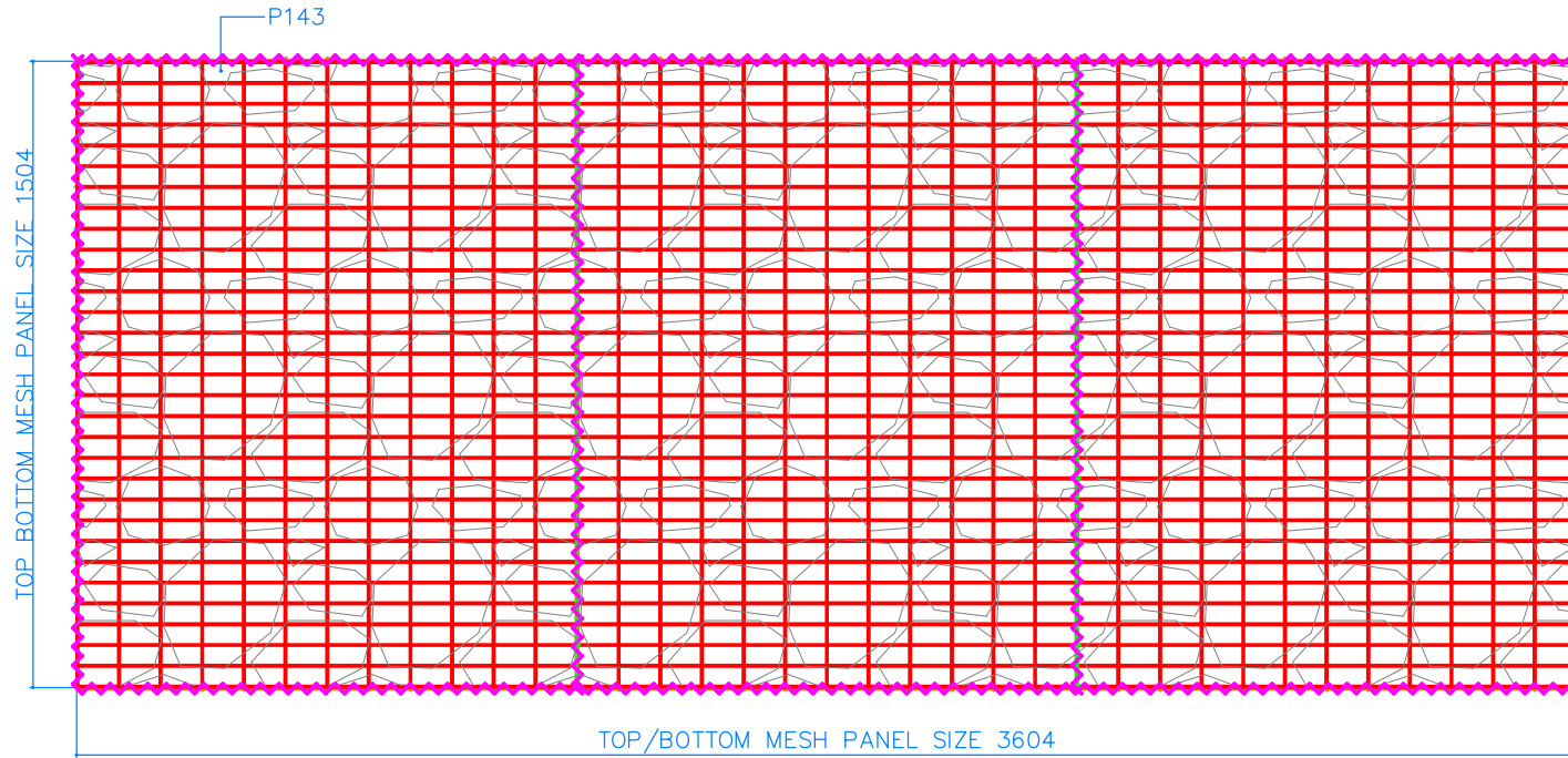
PLAN /TOP
