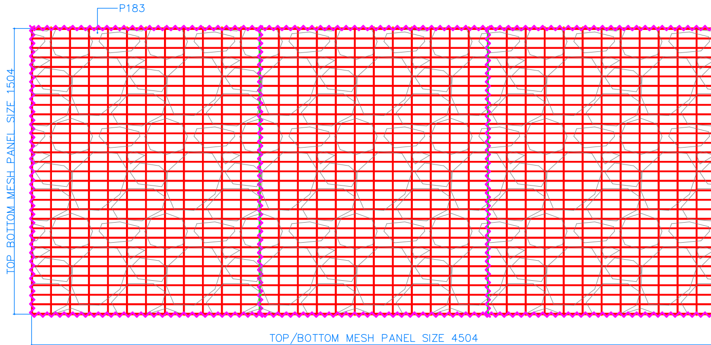
PLAN /TOP
