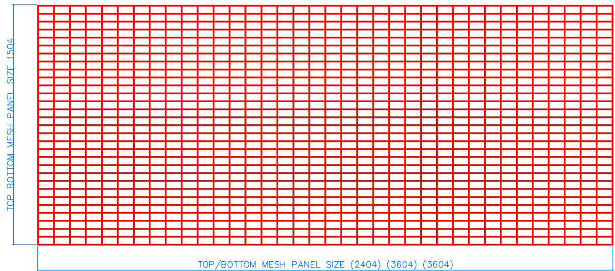
P153 TOP/BOTTOM MESH PANEL QTY-02 MESH SIZE 100X50 WIRE DIA 4MM
