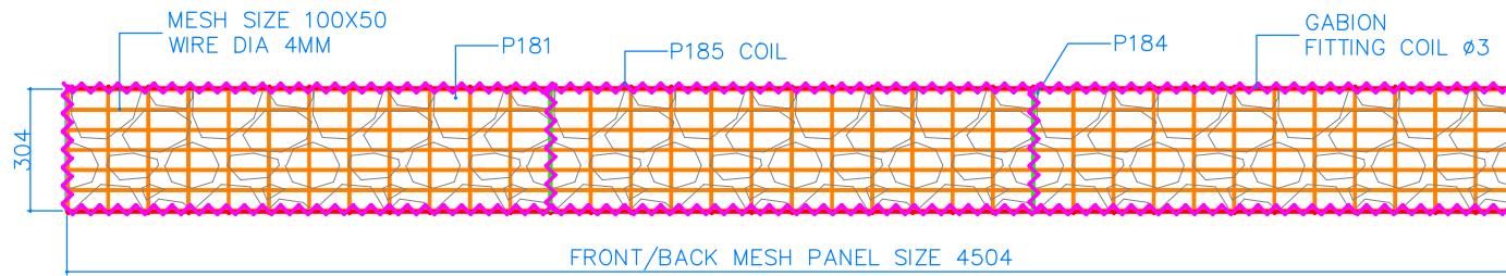
ELEVATION FRONT
