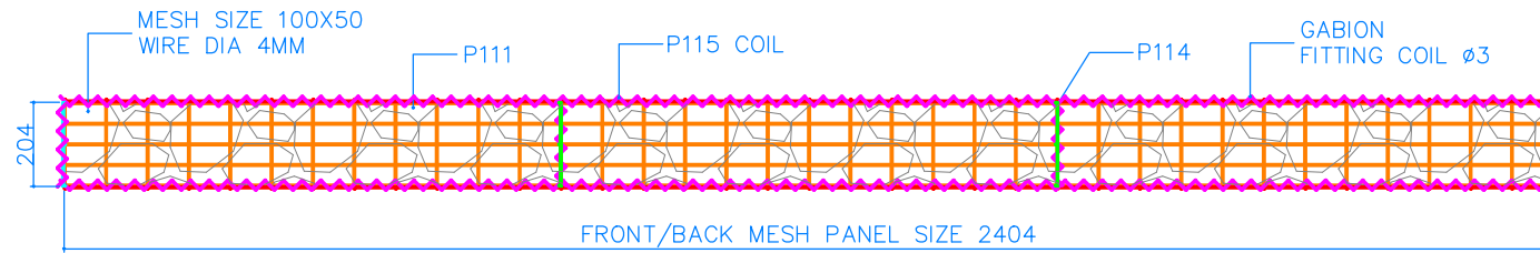
ELEVATION FRONT
