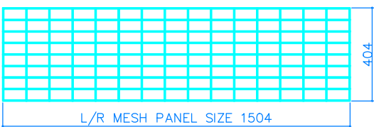
P162 LEFT/RIGHT MESH PANEL QTY-02 MESH SIZE 100X50 WIRE DIA 4MM
