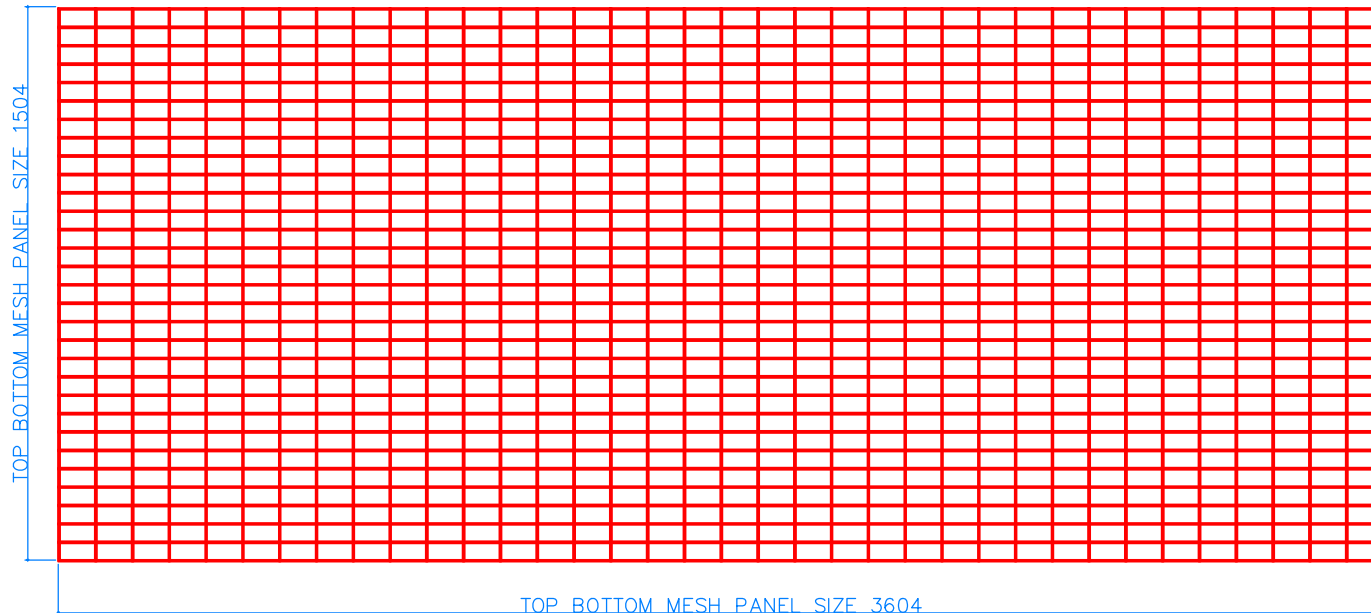
TOP BOTTOM MESH PANEL SIZE 3604
