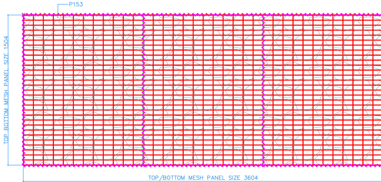
PLAN /TOP
