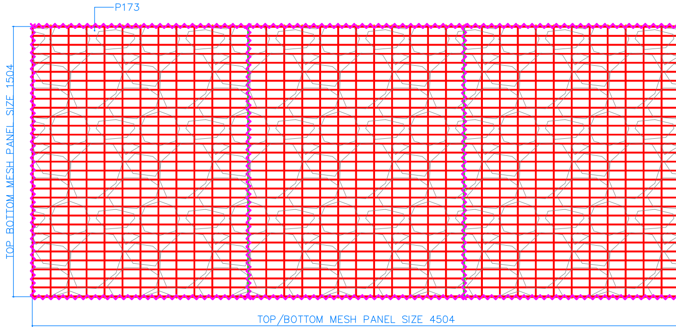
PLAN /TOP
