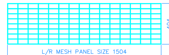
P132 LEFT/RIGHT MESH PANEL QTY-02 MESH SIZE 100X50 WIRE DIA 4MM
