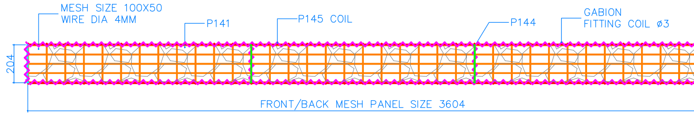
ELEVATION FRONT
