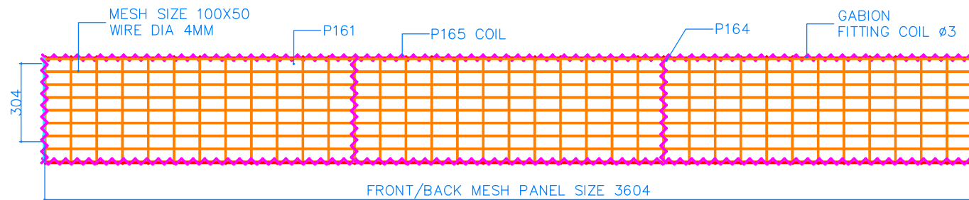
ELEVATION FRONT
