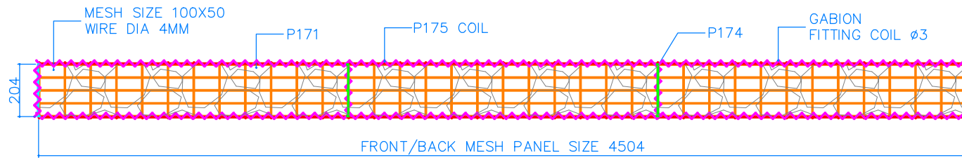
ELEVATION FRONT
