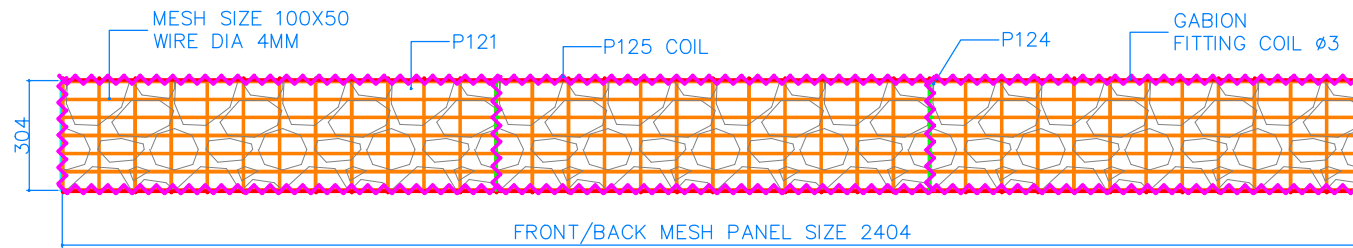
ELEVATION FRONT
