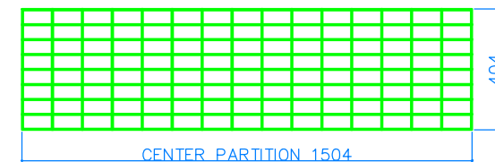
P134 CENTER PARTITION MESH PANEL QTY-03 MESH SIZE 100X50 WIRE DIA 4MM
