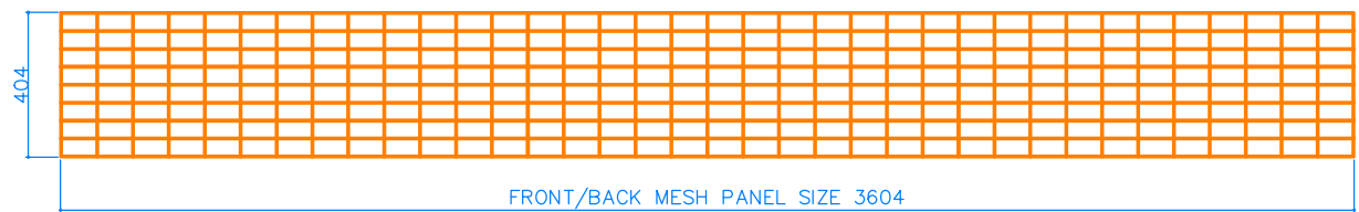
P161 FRONT/BACK MESH PANEL QTY-02 MESH SIZE 100X50 WIRE DIA 4MM
