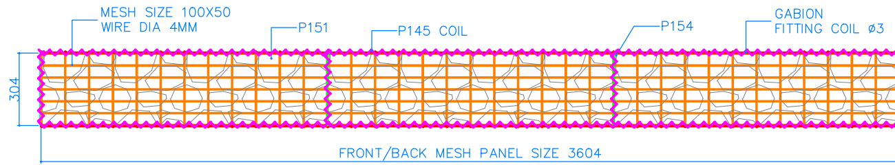
ELEVATION FRONT
