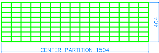
P164 CENTER PARTITION MESH PANEL QTY-03 MESH SIZE 100X50 WIRE DIA 4MM
