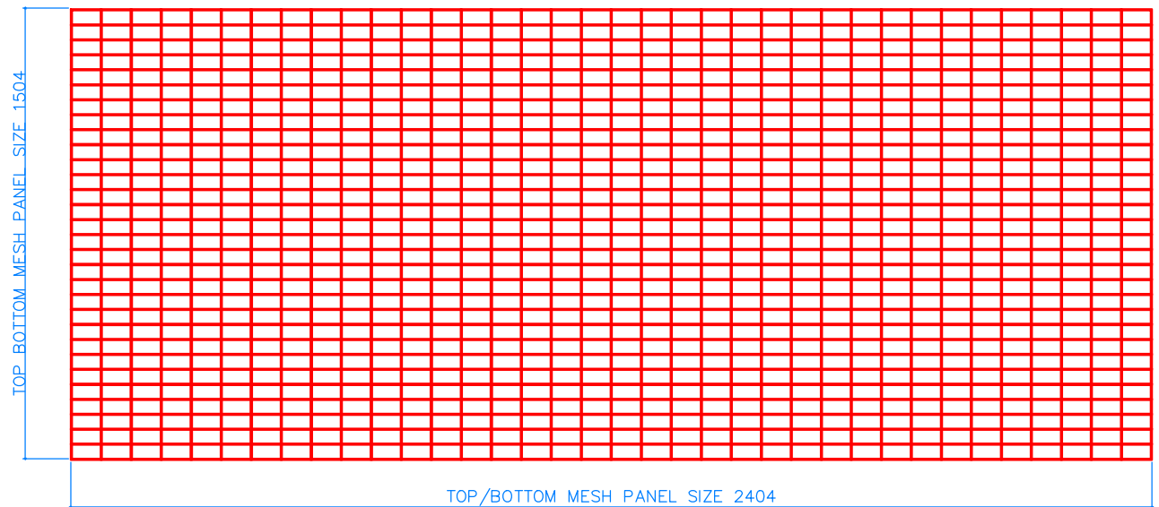
P133 TOP/BOTTOM MESH PANEL QTY-02 MESH SIZE 100X50 WIRE DIA 4MM
