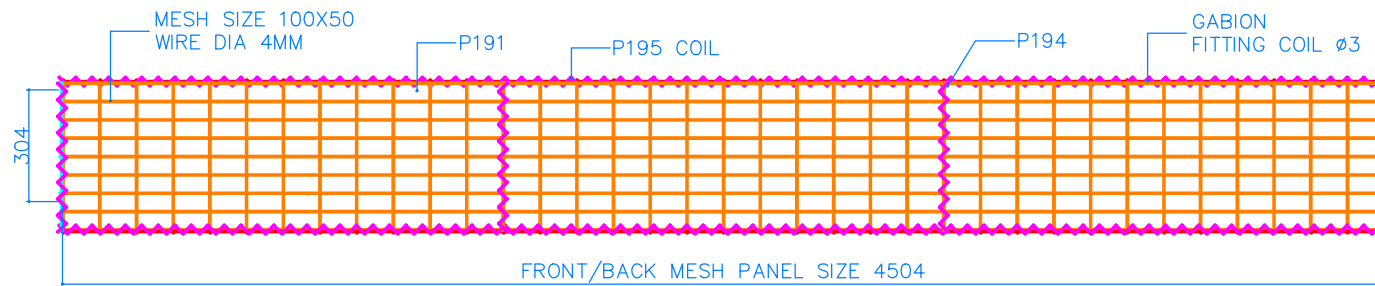
ELEVATION FRONT
