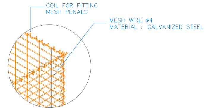
FITTING DETAIL
