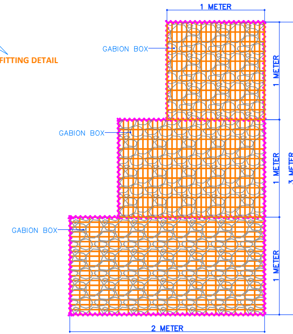
SIDE SECTION
