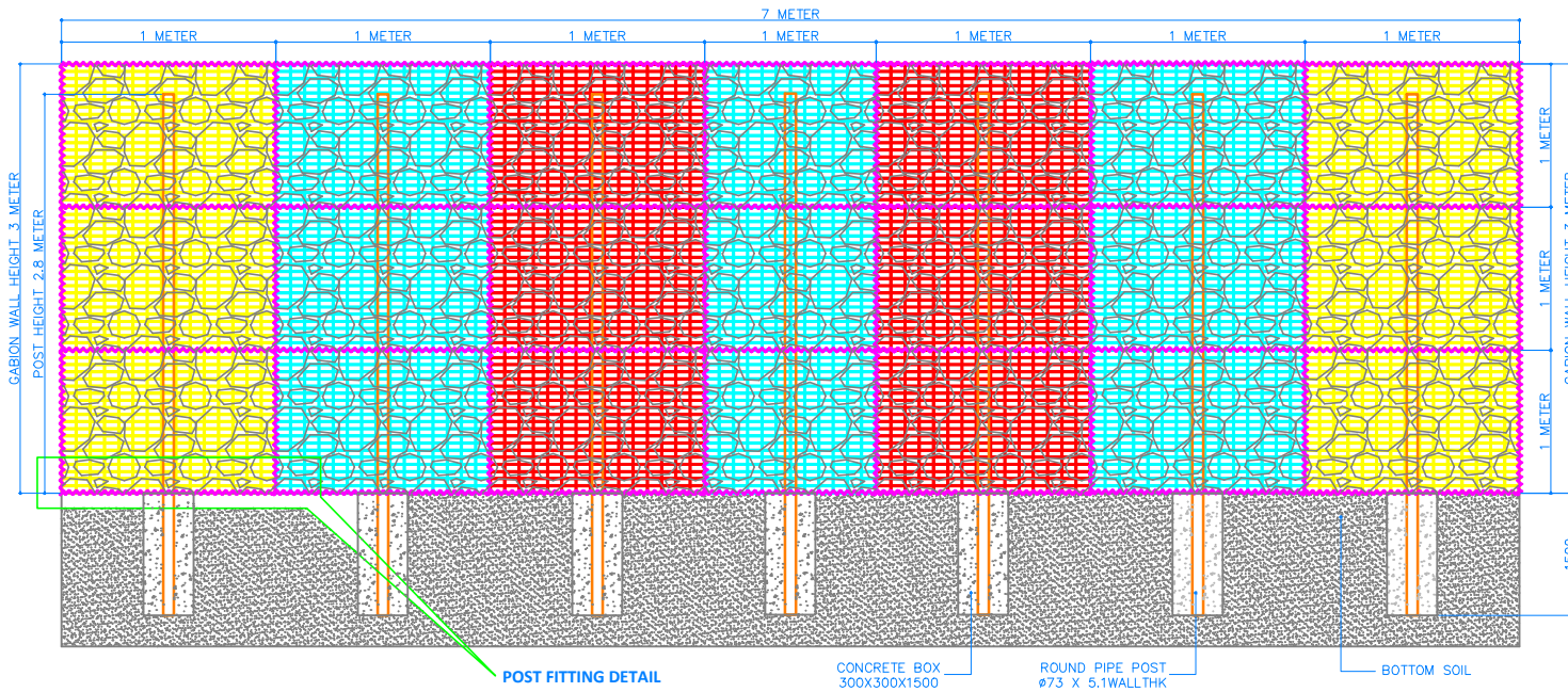
ELEVATION WALL
